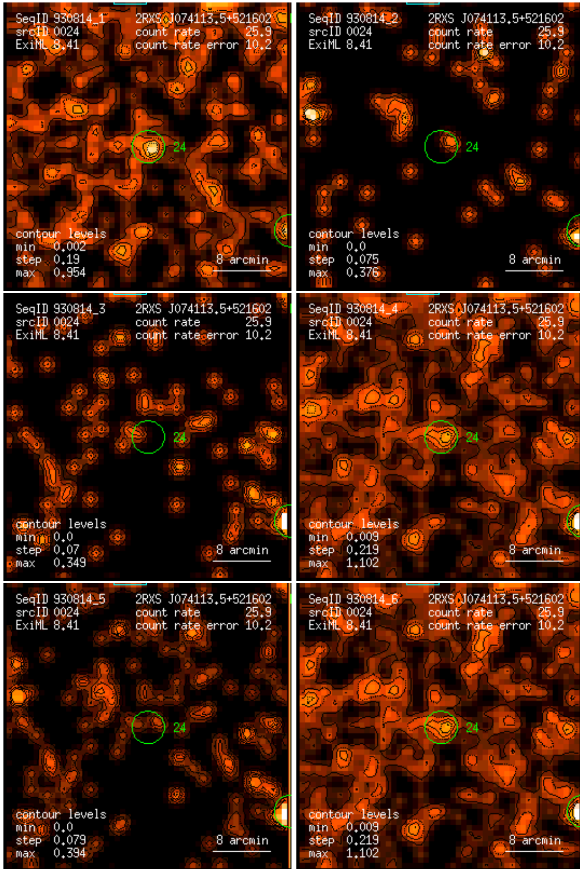
Figure 24: RASS 930814: detection 0024: band rate images, Gaussian filter: (1) PSPC channels 11 – 41, (2) 52 – 90, (3) 91 – 201, (4) 11 – 235, (5) 52 – 201, (6) 11 – 201. Broad band rates in counts/ks. Band rate contour levels in counts/ks/arcmin 2 .
