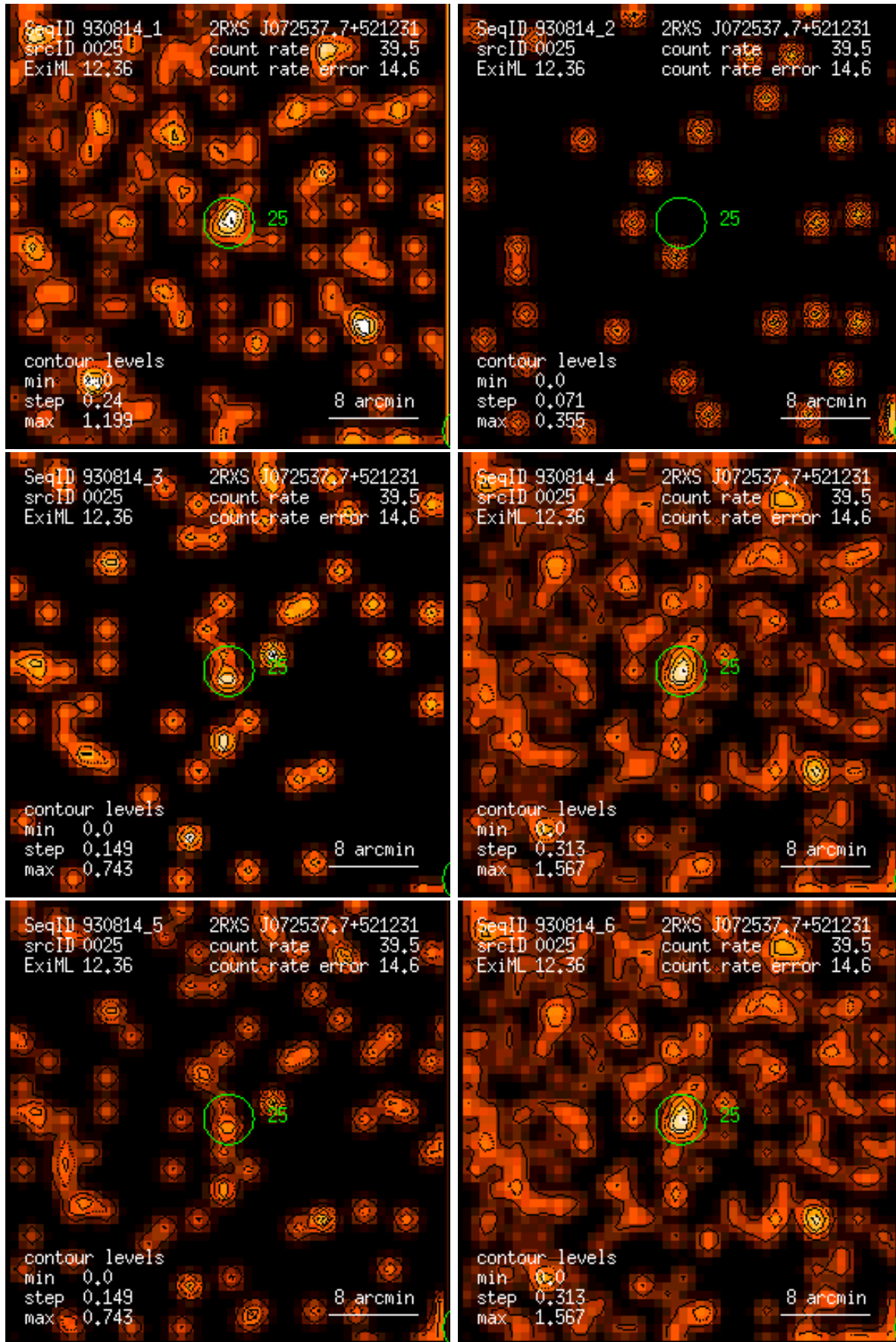
Figure 25: RASS 930814: detection 0025: band rate images, Gaussian filter: (1) PSPC channels 11 – 41, (2) 52 – 90, (3) 91 – 201, (4) 11 – 235, (5) 52 – 201, (6) 11 – 201. Broad band rates in counts/ks. Band rate contour levels in counts/ks/arcmin 2 .
