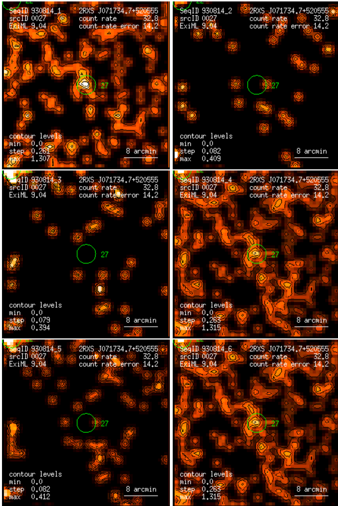
Figure 27: RASS 930814: detection 0027: band rate images, Gaussian filter: (1) PSPC channels 11 – 41, (2) 52 – 90, (3) 91 – 201, (4) 11 – 235, (5) 52 – 201, (6) 11 – 201. Broad band rates in counts/ks. Band rate contour levels in counts/ks/arcmin 2 .
