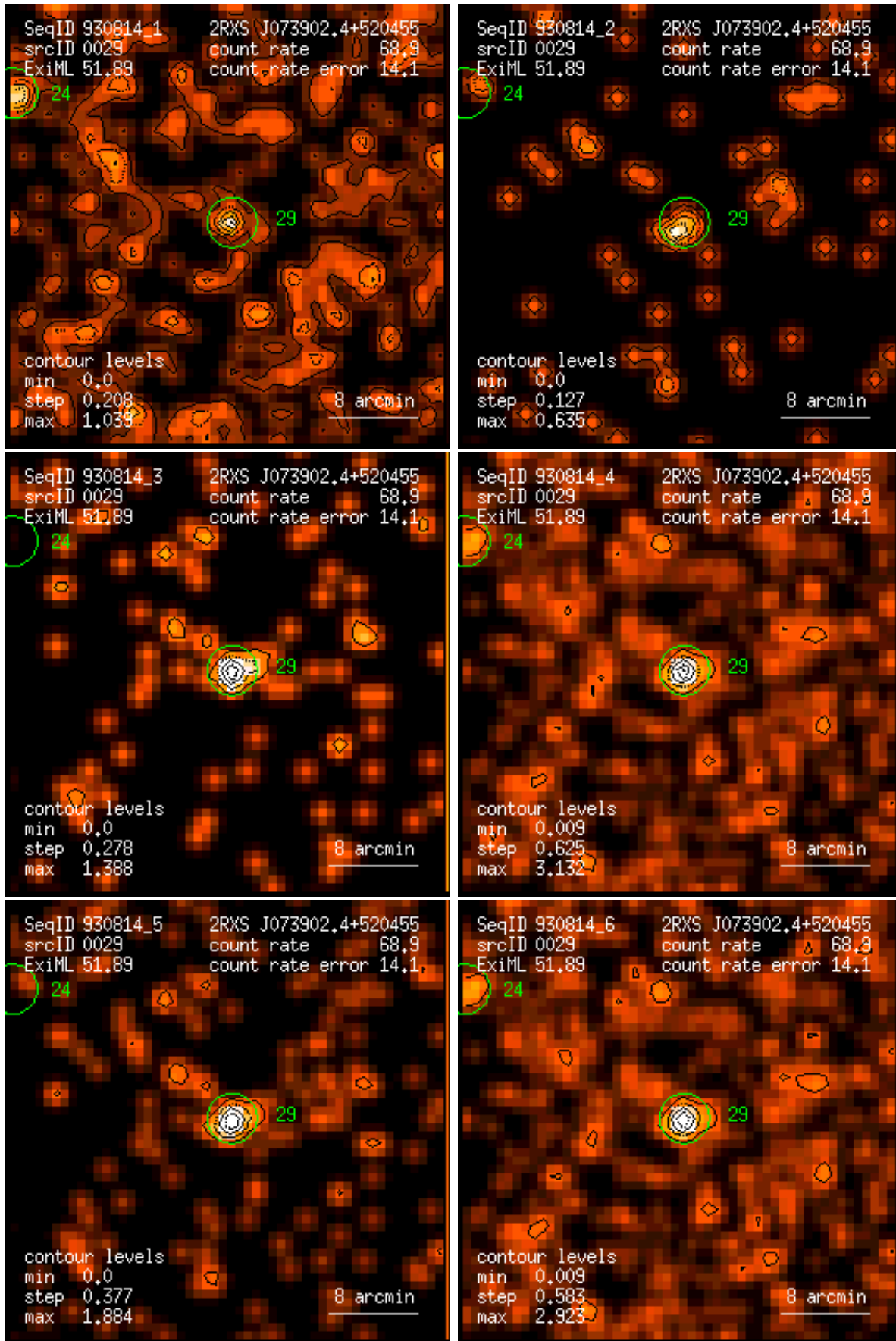
Figure 29: RASS 930814: detection 0029: band rate images, Gaussian filter: (1) PSPC channels 11 – 41, (2) 52 – 90, (3) 91 – 201, (4) 11 – 235, (5) 52 – 201, (6) 11 – 201. Broad band rates in counts/ks. Band rate contour levels in counts/ks/arcmin 2 .
