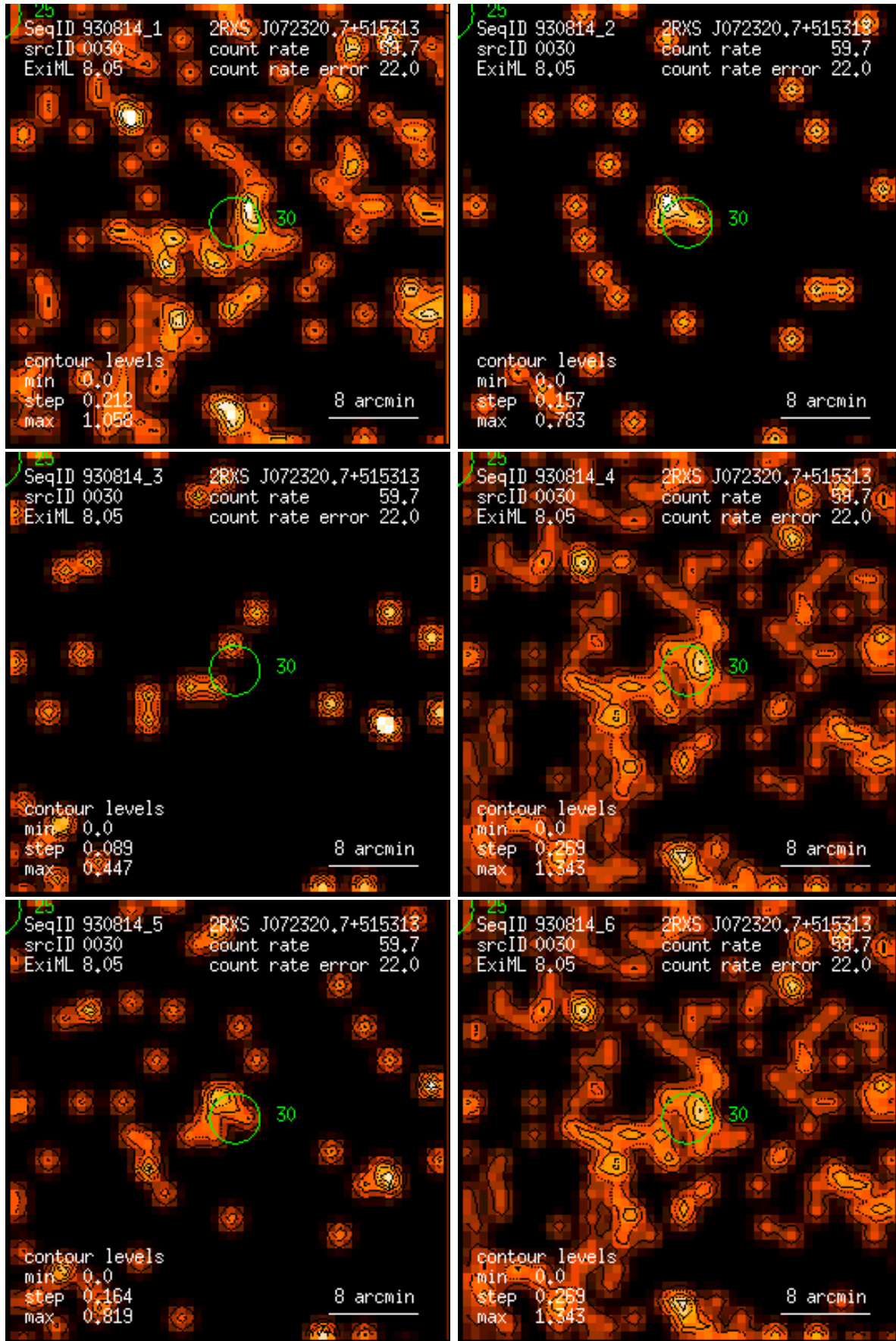
Figure 30: RASS 930814: detection 0030: band rate images, Gaussian filter: (1) PSPC channels 11 – 41, (2) 52 – 90, (3) 91 – 201, (4) 11 – 235, (5) 52 – 201, (6) 11 – 201. Broad band rates in counts/ks. Band rate contour levels in counts/ks/arcmin 2 .
