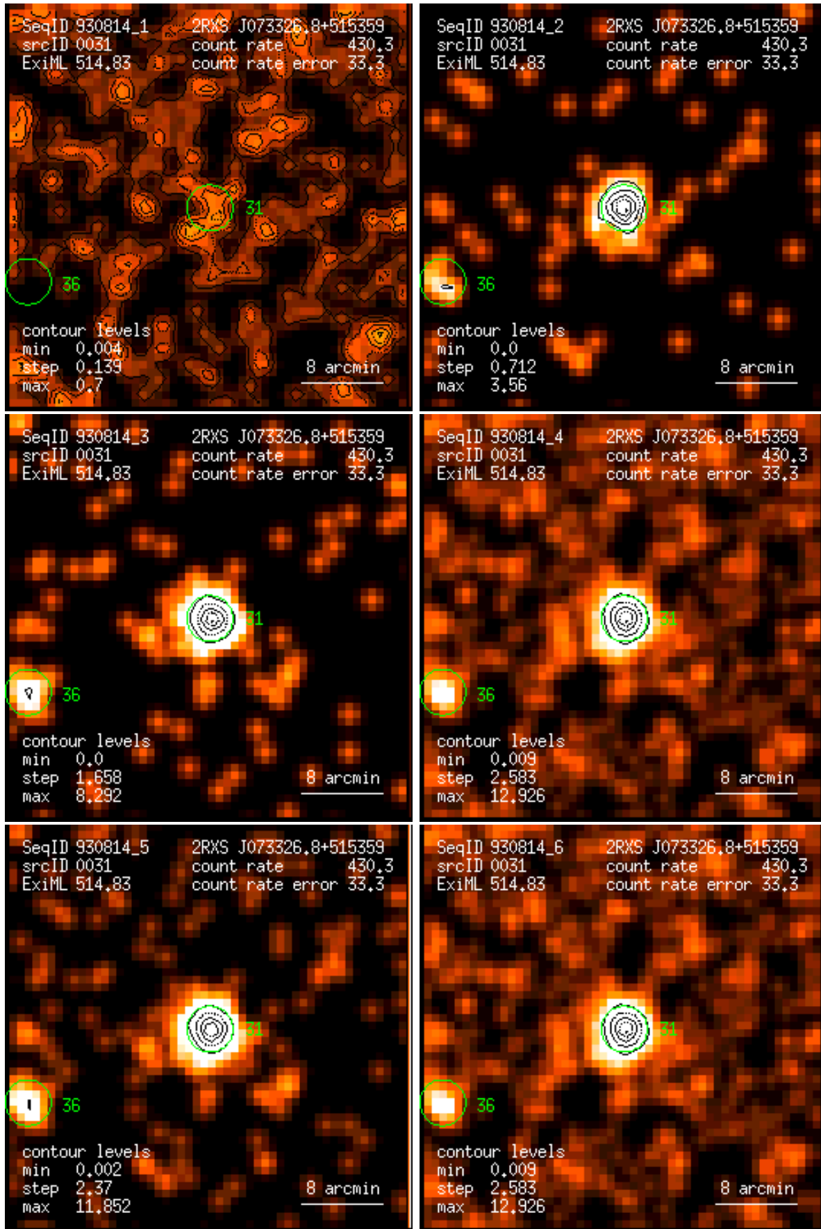
Figure 31: RASS 930814: detection 0031: band rate images, Gaussian filter: (1) PSPC channels 11 – 41, (2) 52 – 90, (3) 91 – 201, (4) 11 – 235, (5) 52 – 201, (6) 11 – 201. Broad band rates in counts/ks. Band rate contour levels in counts/ks/arcmin 2 .
