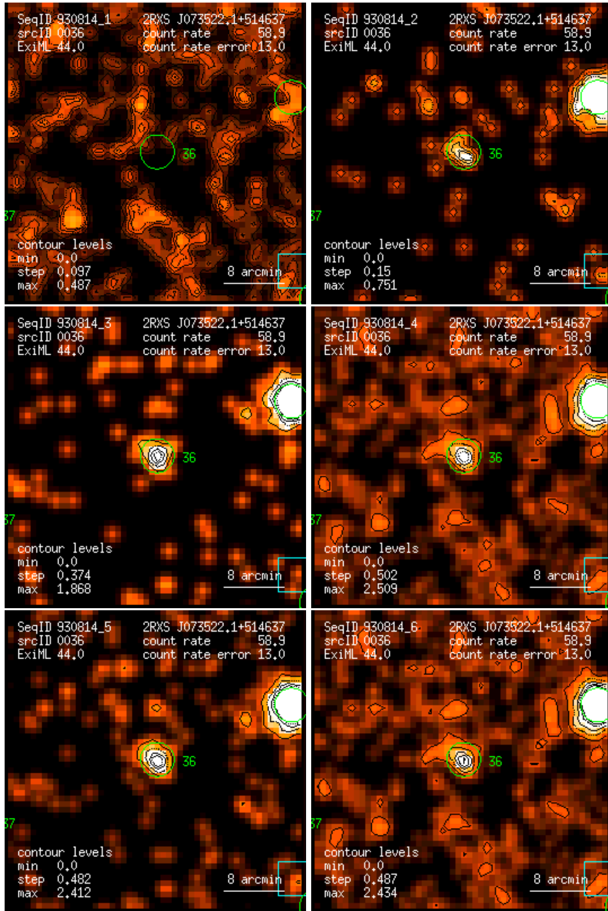
Figure 36: RASS 930814: detection 0036: band rate images, Gaussian filter: (1) PSPC channels 11 – 41, (2) 52 – 90, (3) 91 – 201, (4) 11 – 235, (5) 52 – 201, (6) 11 – 201. Broad band rates in counts/ks. Band rate contour levels in counts/ks/arcmin 2 .
