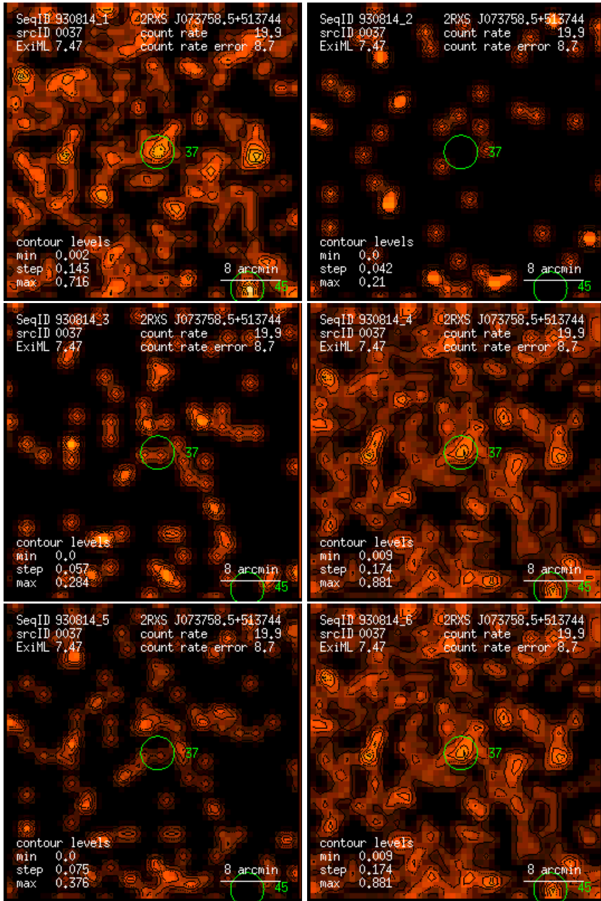
Figure 37: RASS 930814: detection 0037: band rate images, Gaussian filter: (1) PSPC channels 11 – 41, (2) 52 – 90, (3) 91 – 201, (4) 11 – 235, (5) 52 – 201, (6) 11 – 201. Broad band rates in counts/ks. Band rate contour levels in counts/ks/arcmin 2 .
