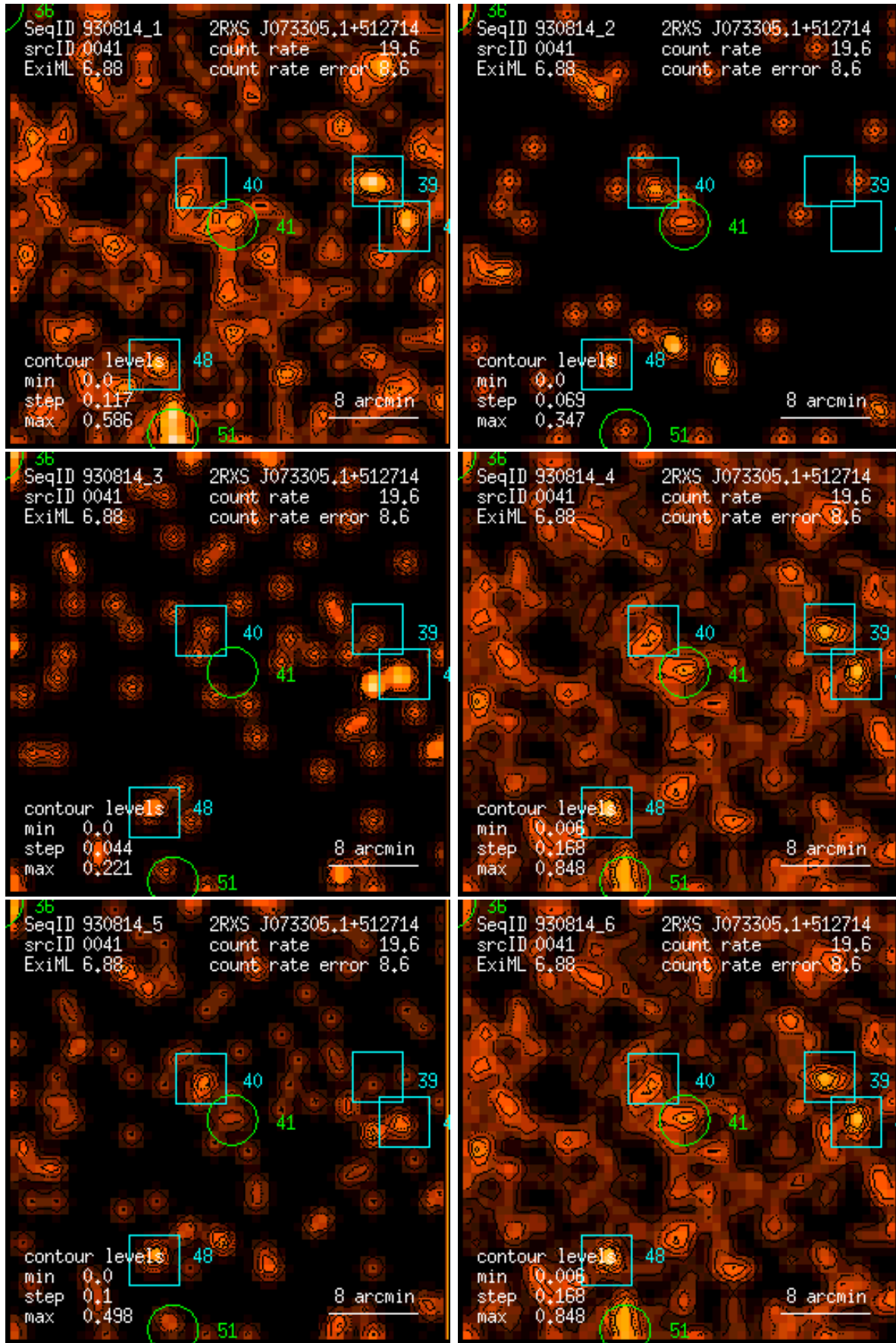
Figure 41: RASS 930814: detection 0041: band rate images, Gaussian filter: (1) PSPC channels 11 – 41, (2) 52 – 90, (3) 91 – 201, (4) 11 – 235, (5) 52 – 201, (6) 11 – 201. Broad band rates in counts/ks. Band rate contour levels in counts/ks/arcmin 2 .
