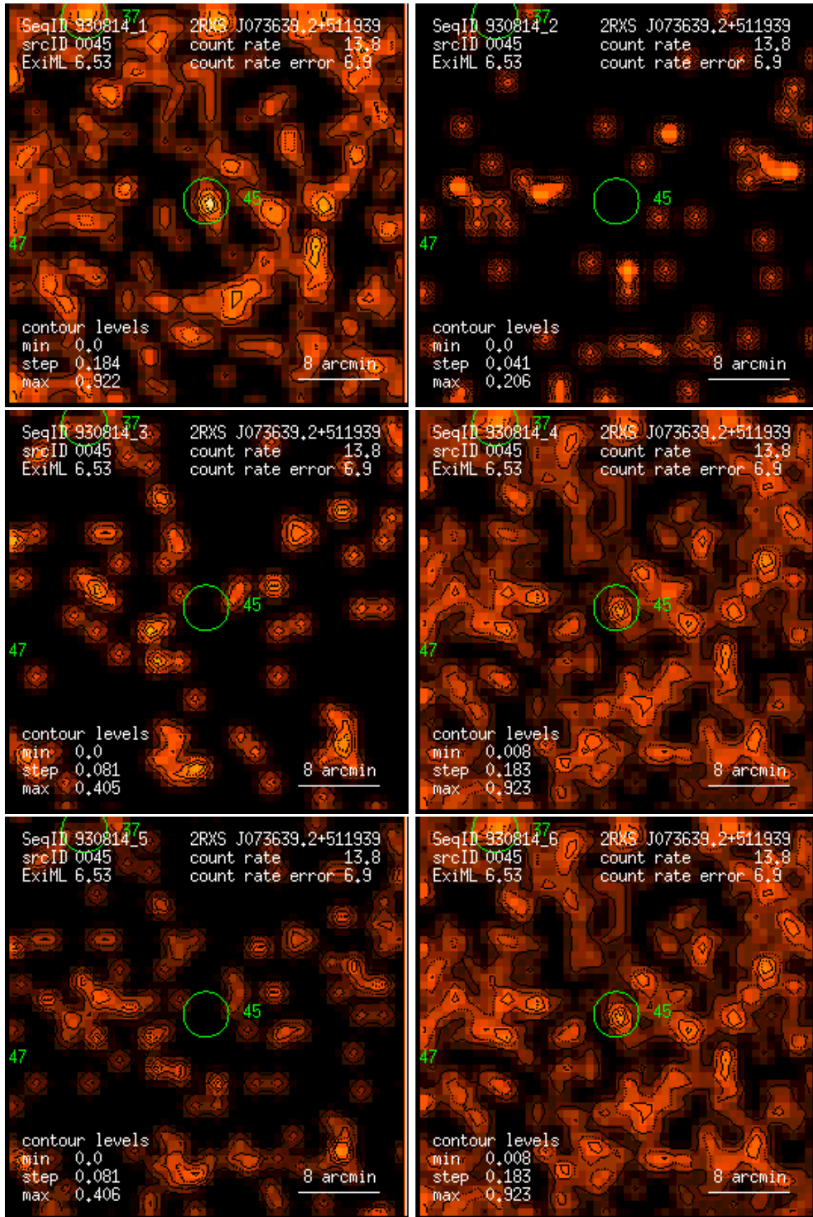
Figure 45: RASS 930814: detection 0045: band rate images, Gaussian filter: (1) PSPC channels 11 – 41, (2) 52 – 90, (3) 91 – 201, (4) 11 – 235, (5) 52 – 201, (6) 11 – 201. Broad band rates in counts/ks. Band rate contour levels in counts/ks/arcmin 2 .
