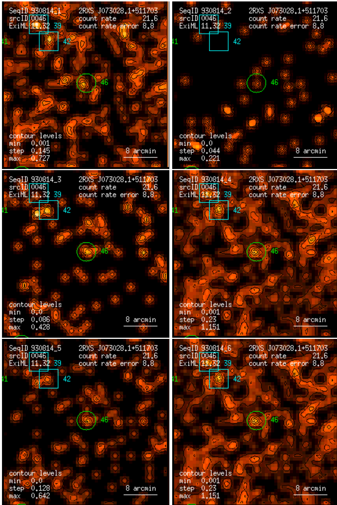
Figure 46: RASS 930814: detection 0046: band rate images, Gaussian filter: (1) PSPC channels 11 – 41, (2) 52 – 90, (3) 91 – 201, (4) 11 – 235, (5) 52 – 201, (6) 11 – 201. Broad band rates in counts/ks. Band rate contour levels in counts/ks/arcmin 2 .
