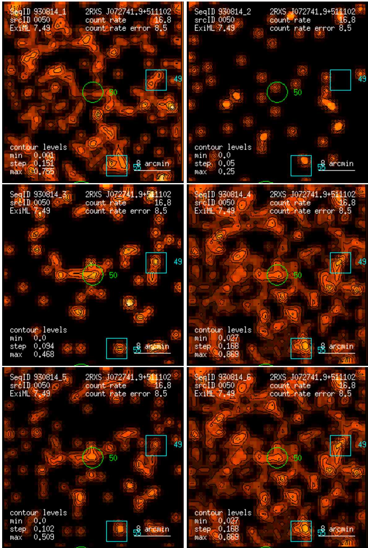
Figure 50: RASS 930814: detection 0050: band rate images, Gaussian filter: (1) PSPC channels 11 – 41, (2) 52 – 90, (3) 91 – 201, (4) 11 – 235, (5) 52 – 201, (6) 11 – 201. Broad band rates in counts/ks. Band rate contour levels in counts/ks/arcmin 2 .
