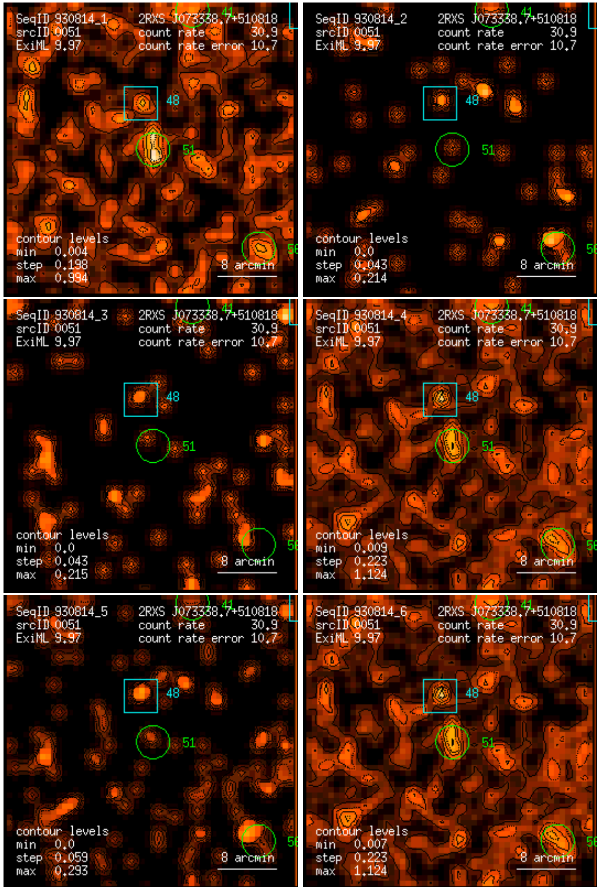
Figure 51: RASS 930814: detection 0051: band rate images, Gaussian filter: (1) PSPC channels 11 – 41, (2) 52 – 90, (3) 91 – 201, (4) 11 – 235, (5) 52 – 201, (6) 11 – 201. Broad band rates in counts/ks. Band rate contour levels in counts/ks/arcmin 2 .
