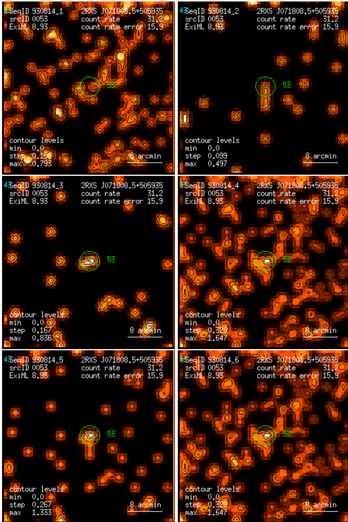
Figure 53: RASS 930814: detection 0053: band rate images, Gaussian filter: (1) PSPC channels 11 – 41, (2) 52 – 90, (3) 91 – 201, (4) 11 – 235, (5) 52 – 201, (6) 11 – 201. Broad band rates in counts/ks. Band rate contour levels in counts/ks/arcmin 2 .
