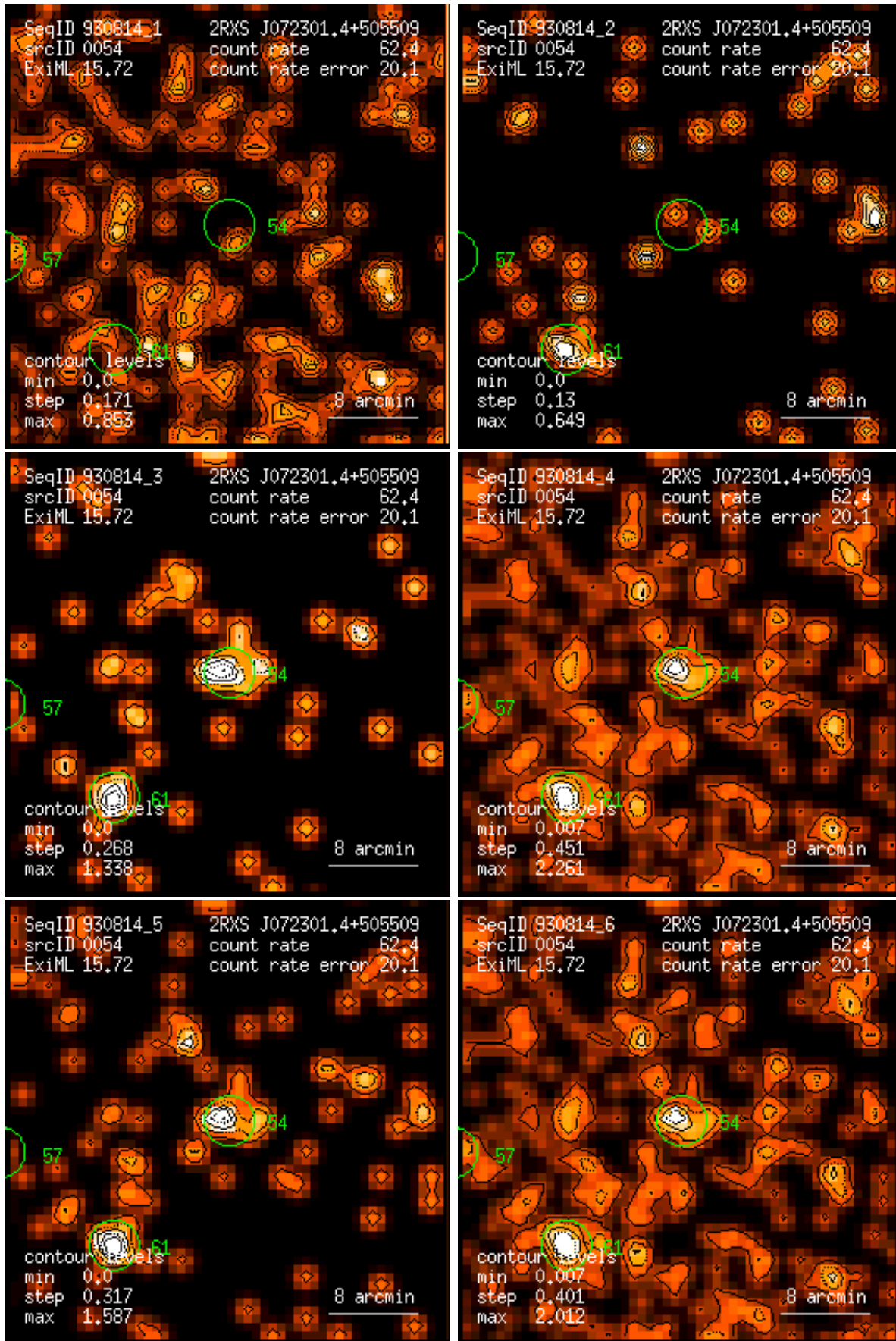
Figure 54: RASS 930814: detection 0054: band rate images, Gaussian filter: (1) PSPC channels 11 – 41, (2) 52 – 90, (3) 91 – 201, (4) 11 – 235, (5) 52 – 201, (6) 11 – 201. Broad band rates in counts/ks. Band rate contour levels in counts/ks/arcmin 2 .
