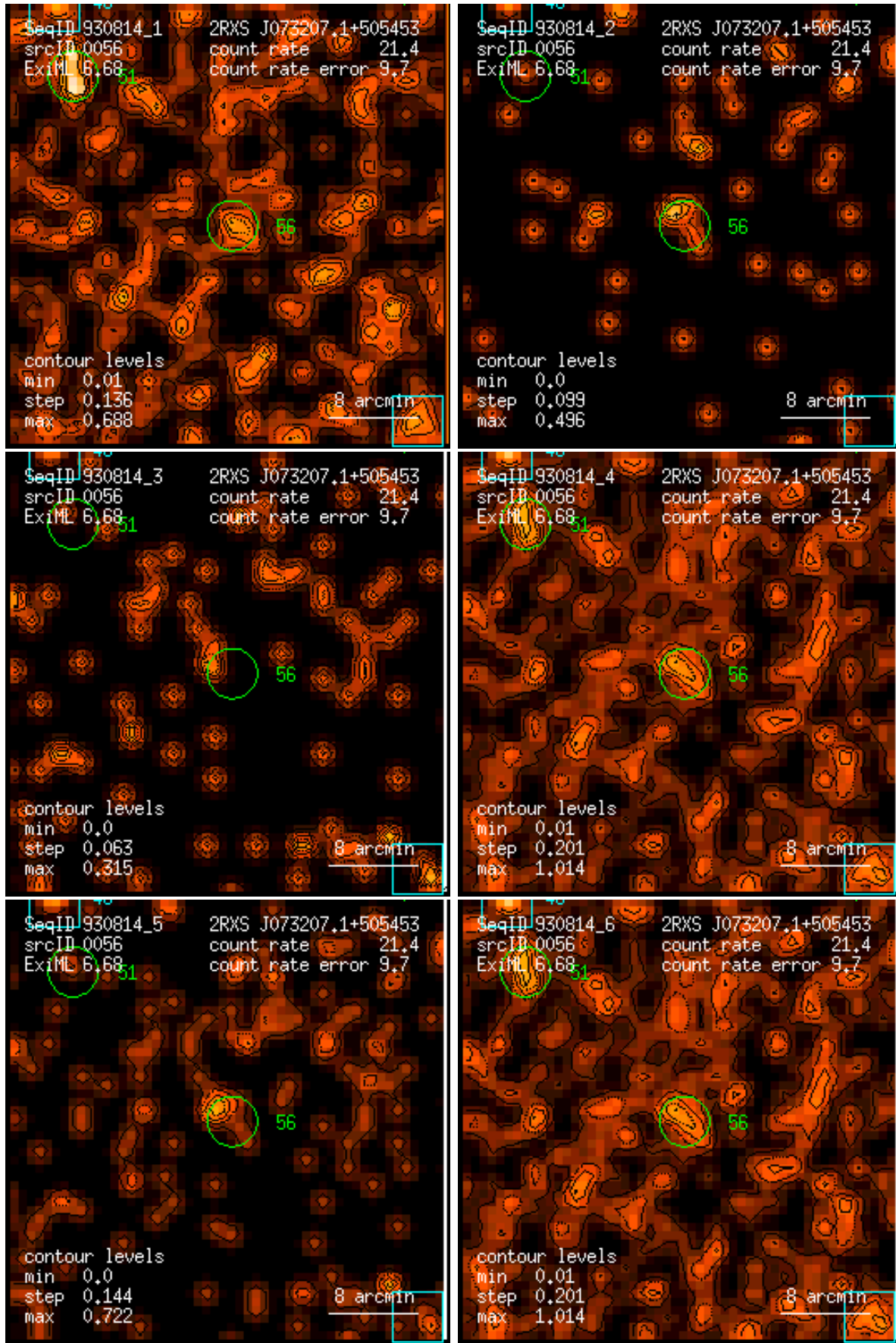
Figure 56: RASS 930814: detection 0056: band rate images, Gaussian filter: (1) PSPC channels 11 – 41, (2) 52 – 90, (3) 91 – 201, (4) 11 – 235, (5) 52 – 201, (6) 11 – 201. Broad band rates in counts/ks. Band rate contour levels in counts/ks/arcmin 2 .
