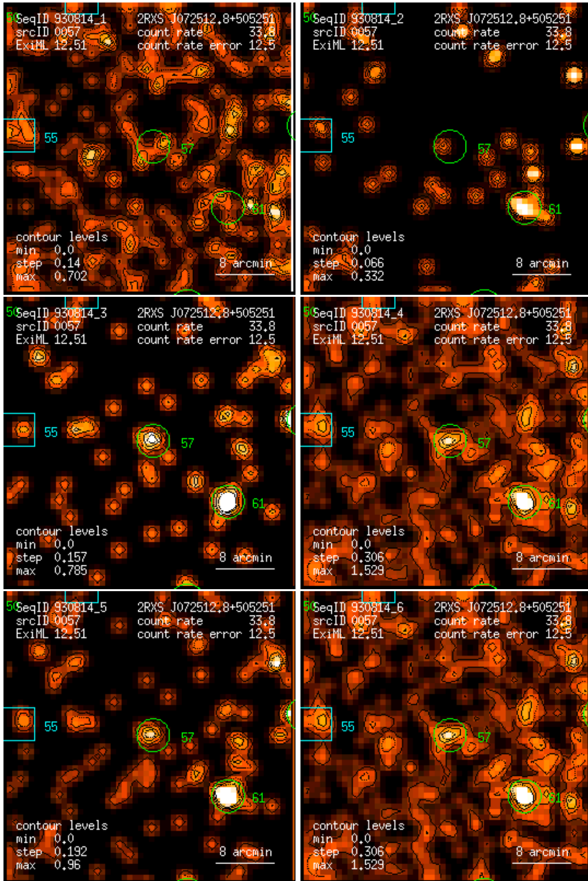
Figure 57: RASS 930814: detection 0057: band rate images, Gaussian filter: (1) PSPC channels 11 – 41, (2) 52 – 90, (3) 91 – 201, (4) 11 – 235, (5) 52 – 201, (6) 11 – 201. Broad band rates in counts/ks. Band rate contour levels in counts/ks/arcmin 2 .
