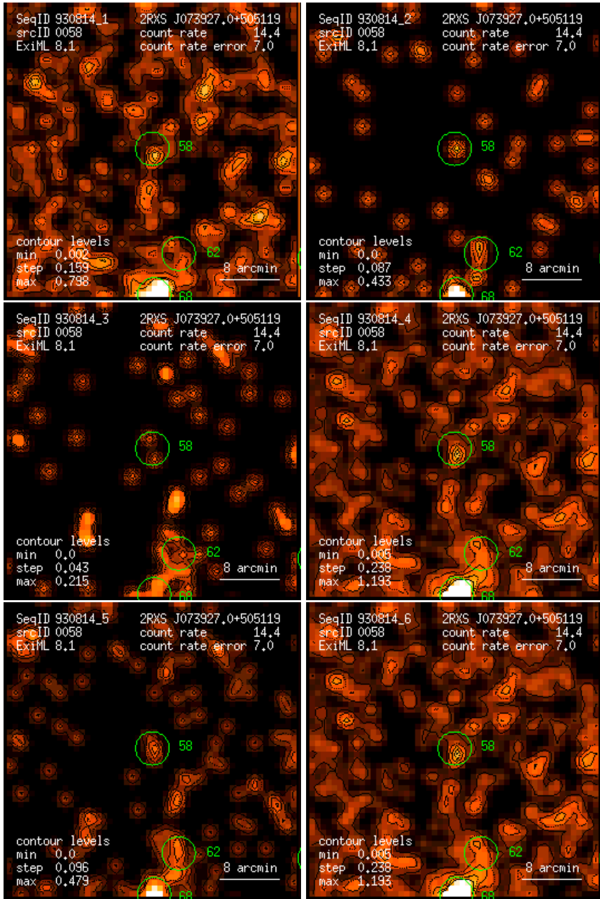
Figure 58: RASS 930814: detection 0058: band rate images, Gaussian filter: (1) PSPC channels 11 – 41, (2) 52 – 90, (3) 91 – 201, (4) 11 – 235, (5) 52 – 201, (6) 11 – 201. Broad band rates in counts/ks. Band rate contour levels in counts/ks/arcmin 2 .
