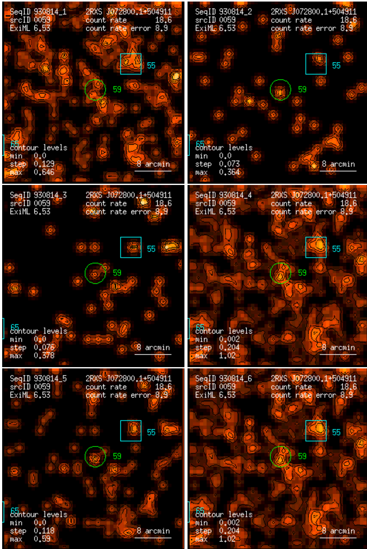
Figure 59: RASS 930814: detection 0059: band rate images, Gaussian filter: (1) PSPC channels 11 – 41, (2) 52 – 90, (3) 91 – 201, (4) 11 – 235, (5) 52 – 201, (6) 11 – 201. Broad band rates in counts/ks. Band rate contour levels in counts/ks/arcmin 2 .
