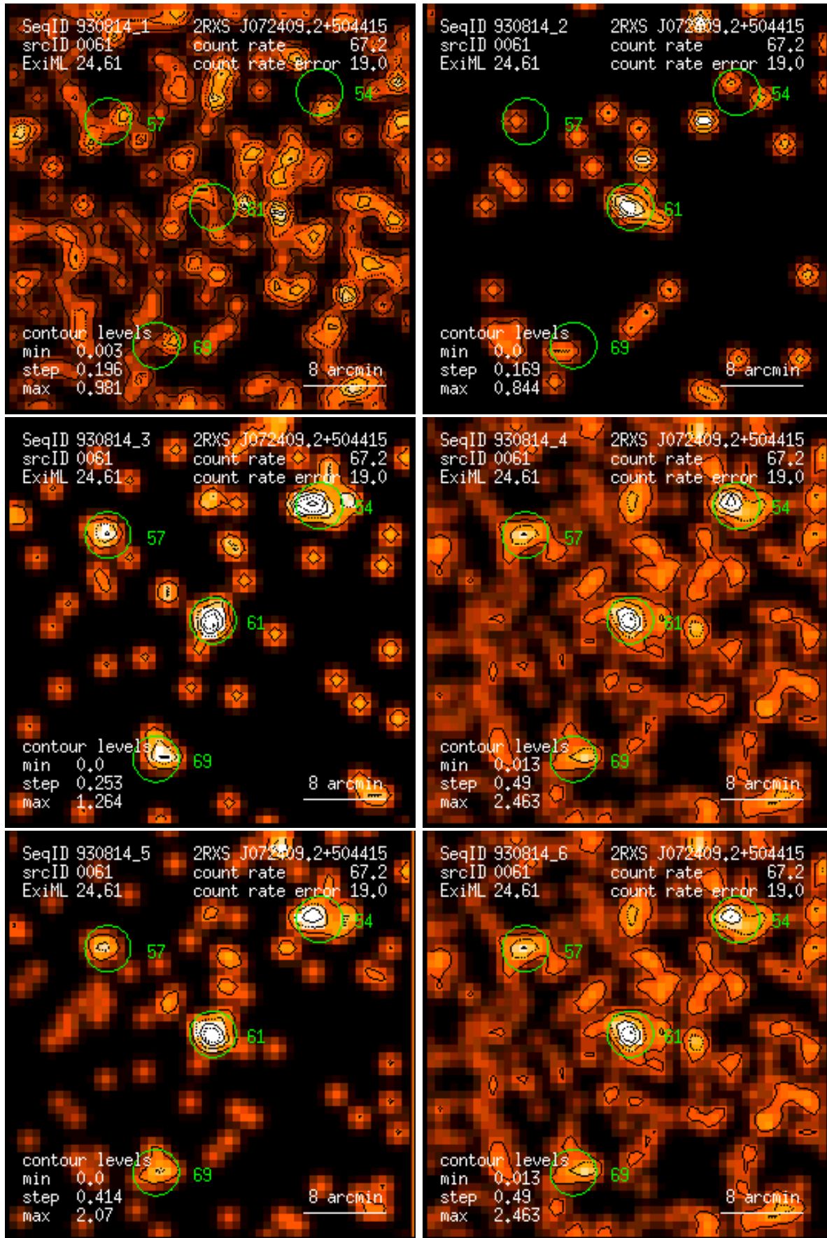
Figure 61: RASS 930814: detection 0061: band rate images, Gaussian filter: (1) PSPC channels 11 – 41, (2) 52 – 90, (3) 91 – 201, (4) 11 – 235, (5) 52 – 201, (6) 11 – 201. Broad band rates in counts/ks. Band rate contour levels in counts/ks/arcmin 2 .
