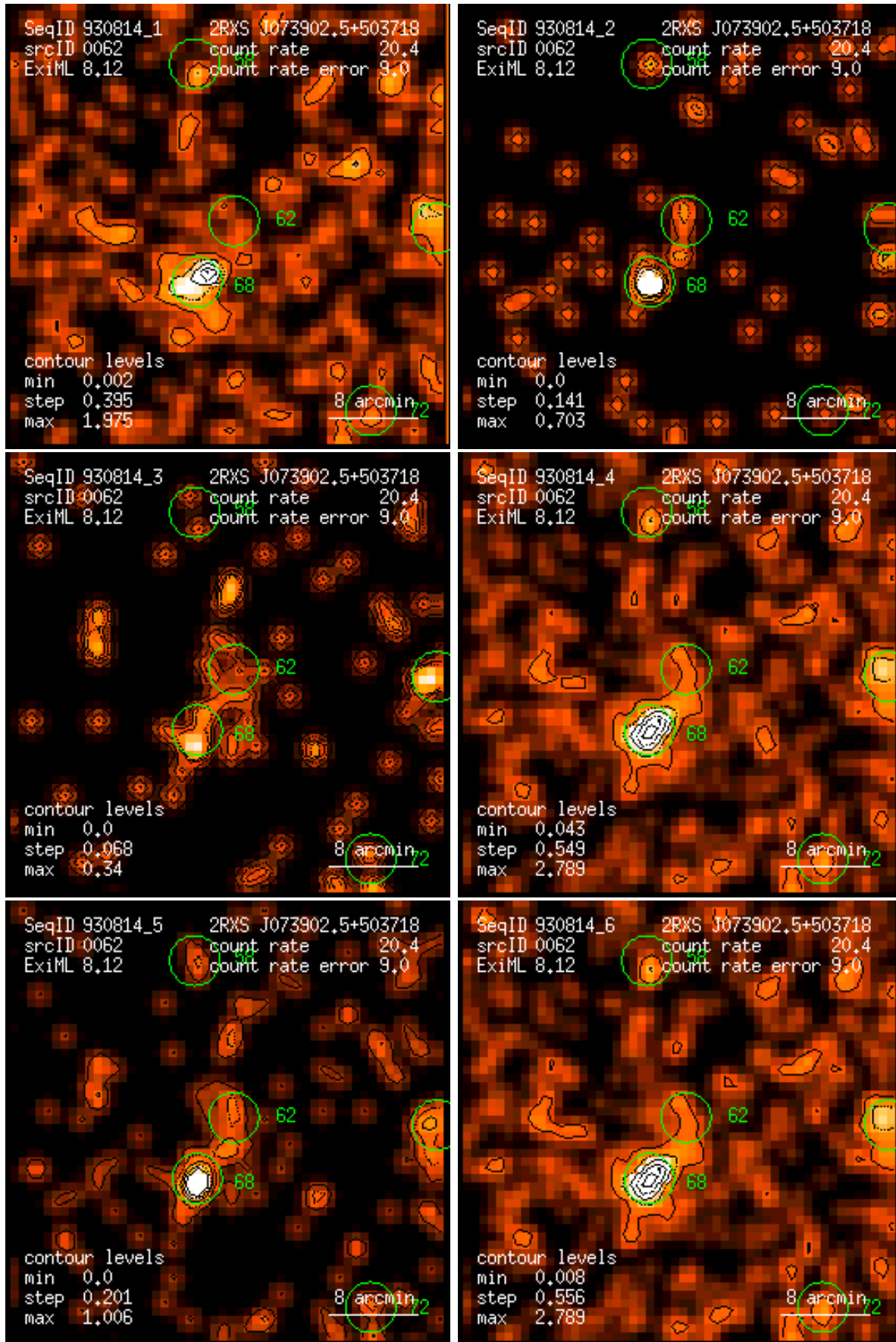
Figure 62: RASS 930814: detection 0062: band rate images, Gaussian filter: (1) PSPC channels 11 – 41, (2) 52 – 90, (3) 91 – 201, (4) 11 – 235, (5) 52 – 201, (6) 11 – 201. Broad band rates in counts/ks. Band rate contour levels in counts/ks/arcmin 2 .
