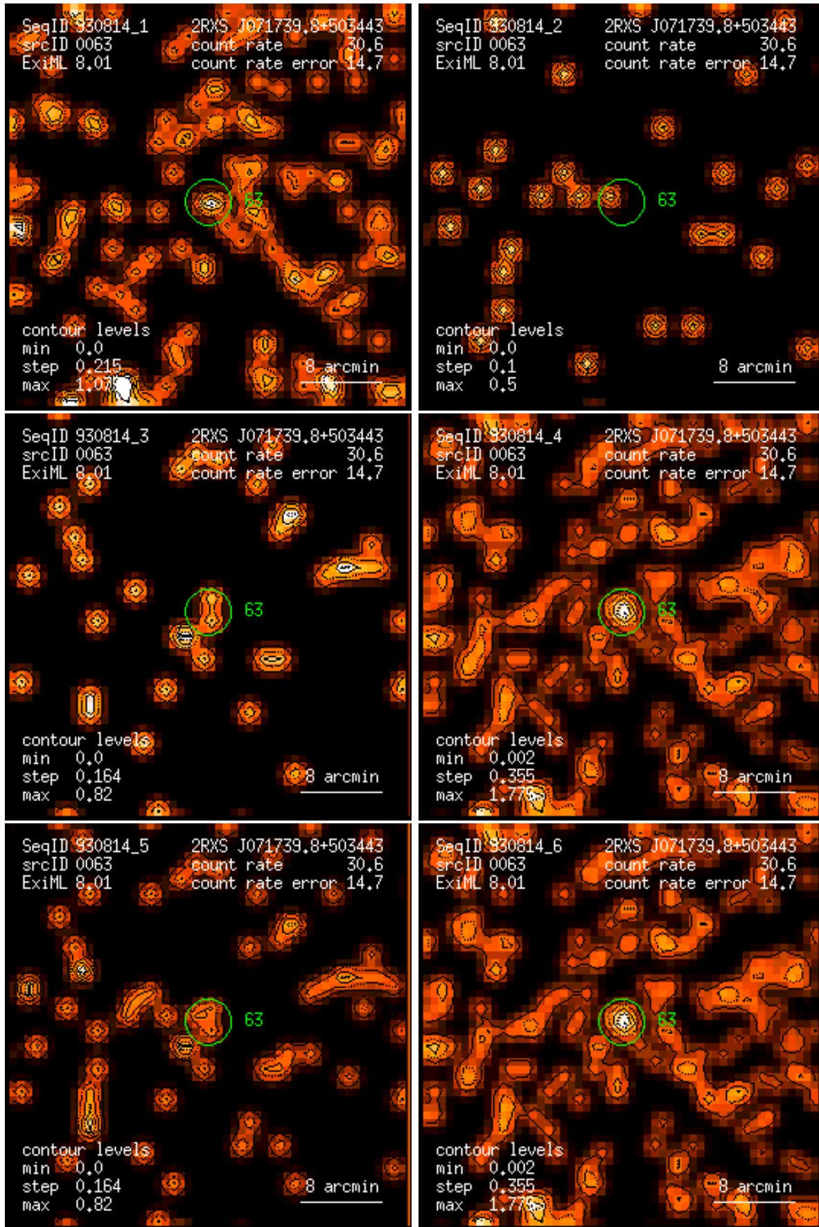
Figure 63: RASS 930814: detection 0063: band rate images, Gaussian filter: (1) PSPC channels 11 – 41, (2) 52 – 90, (3) 91 – 201, (4) 11 – 235, (5) 52 – 201, (6) 11 – 201. Broad band rates in counts/ks. Band rate contour levels in counts/ks/arcmin 2 .
