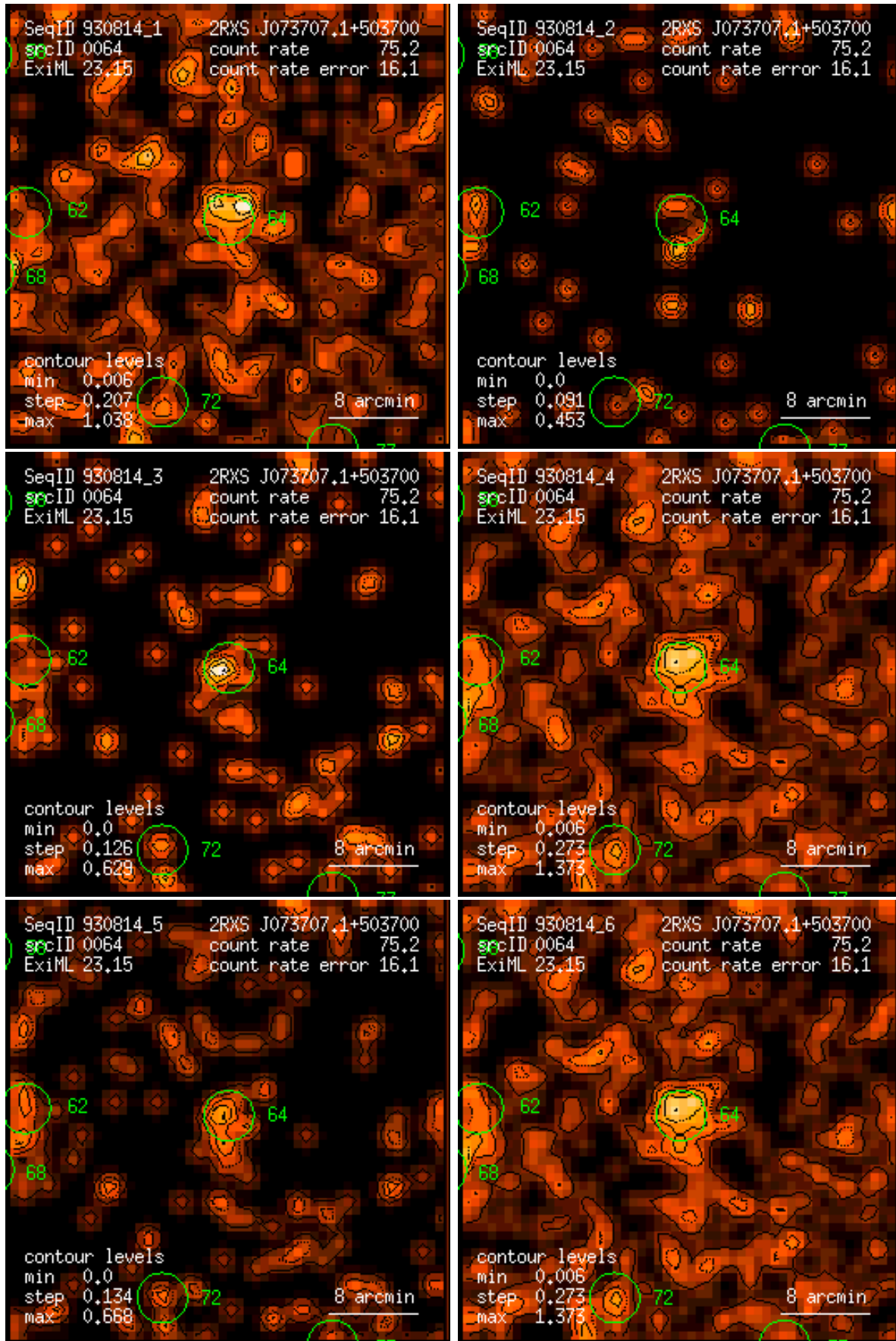
Figure 64: RASS 930814: detection 0064: band rate images, Gaussian filter: (1) PSPC channels 11 – 41, (2) 52 – 90, (3) 91 – 201, (4) 11 – 235, (5) 52 – 201, (6) 11 – 201. Broad band rates in counts/ks. Band rate contour levels in counts/ks/arcmin 2 .
