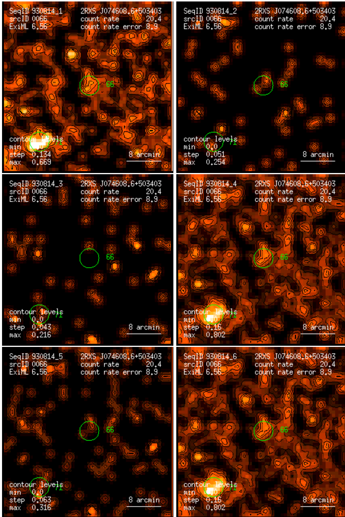
Figure 66: RASS 930814: detection 0066: band rate images, Gaussian filter: (1) PSPC channels 11 – 41, (2) 52 – 90, (3) 91 – 201, (4) 11 – 235, (5) 52 – 201, (6) 11 – 201. Broad band rates in counts/ks. Band rate contour levels in counts/ks/arcmin 2 .
