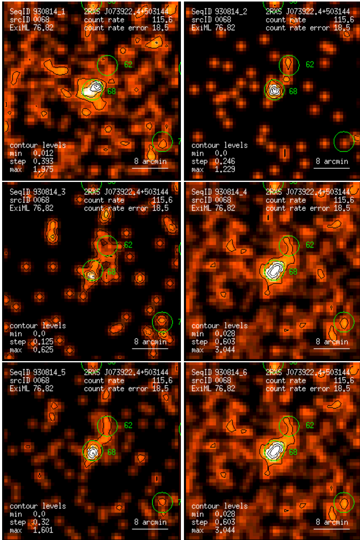
Figure 68: RASS 930814: detection 0068: band rate images, Gaussian filter: (1) PSPC channels 11 – 41, (2) 52 – 90, (3) 91 – 201, (4) 11 – 235, (5) 52 – 201, (6) 11 – 201. Broad band rates in counts/ks. Band rate contour levels in counts/ks/arcmin 2 .
