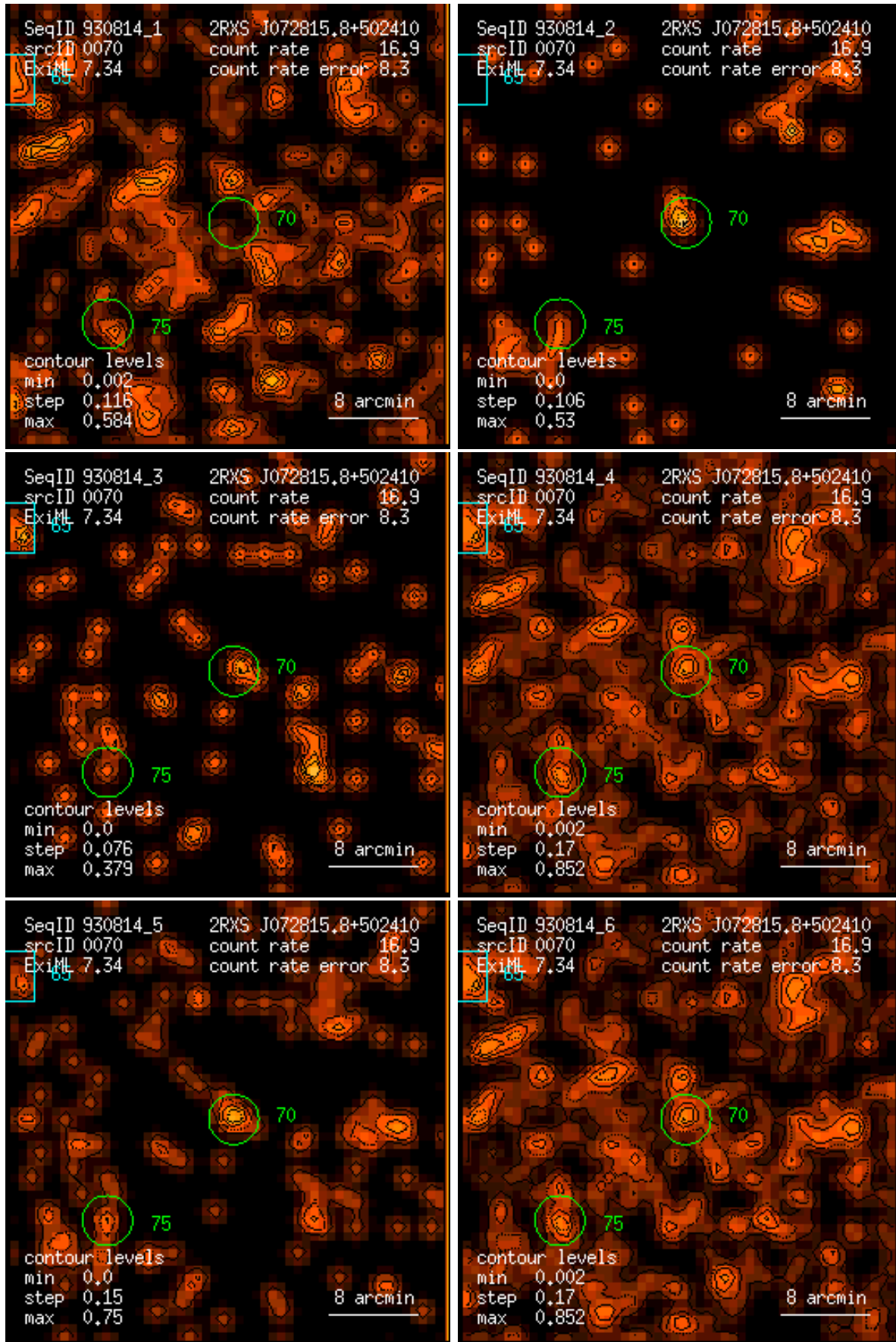
Figure 70: RASS 930814: detection 0070: band rate images, Gaussian filter: (1) PSPC channels 11 – 41, (2) 52 – 90, (3) 91 – 201, (4) 11 – 235, (5) 52 – 201, (6) 11 – 201. Broad band rates in counts/ks. Band rate contour levels in counts/ks/arcmin 2 .
