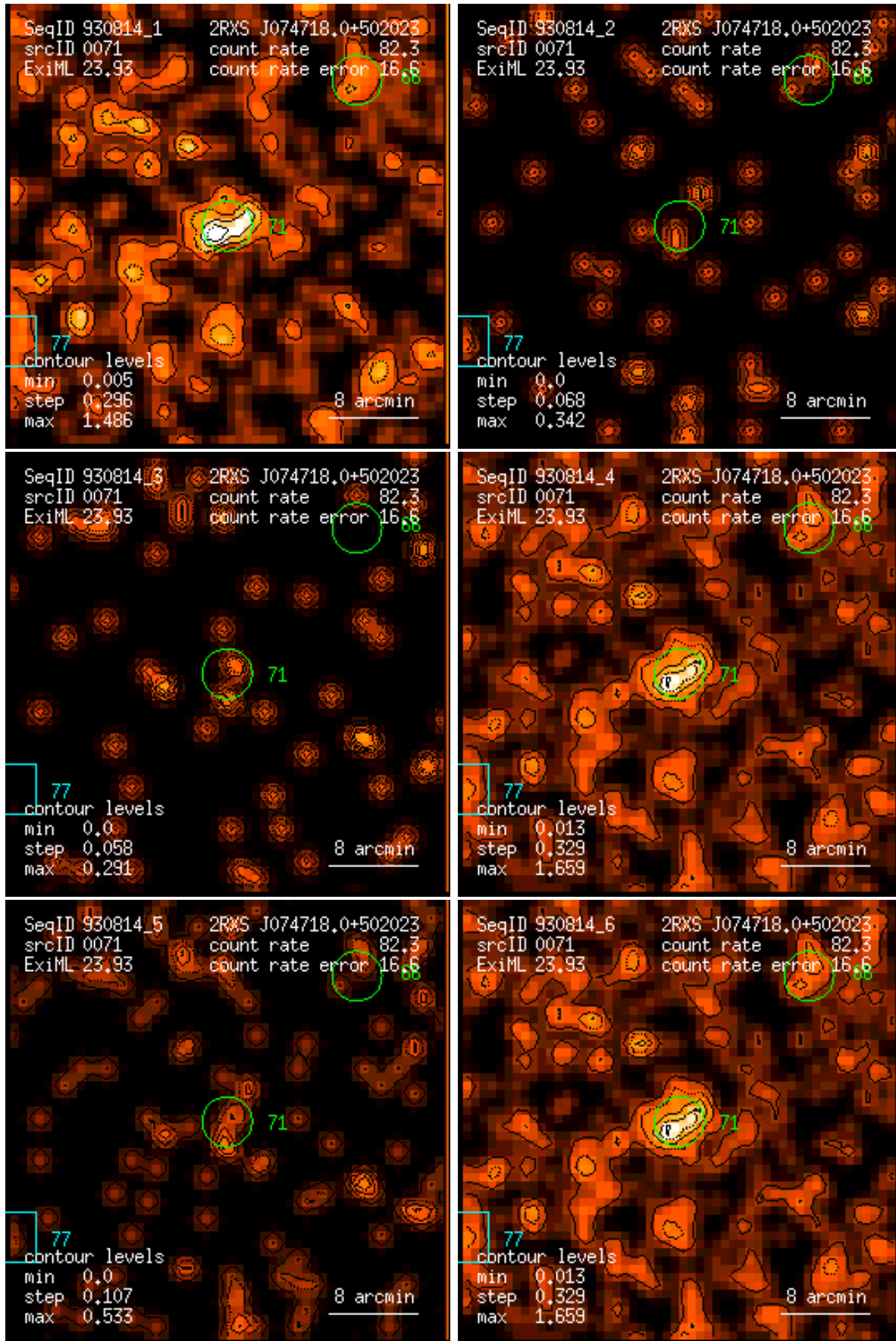
Figure 71: RASS 930814: detection 0071: band rate images, Gaussian filter: (1) PSPC channels 11 – 41, (2) 52 – 90, (3) 91 – 201, (4) 11 – 235, (5) 52 – 201, (6) 11 – 201. Broad band rates in counts/ks. Band rate contour levels in counts/ks/arcmin 2 .
