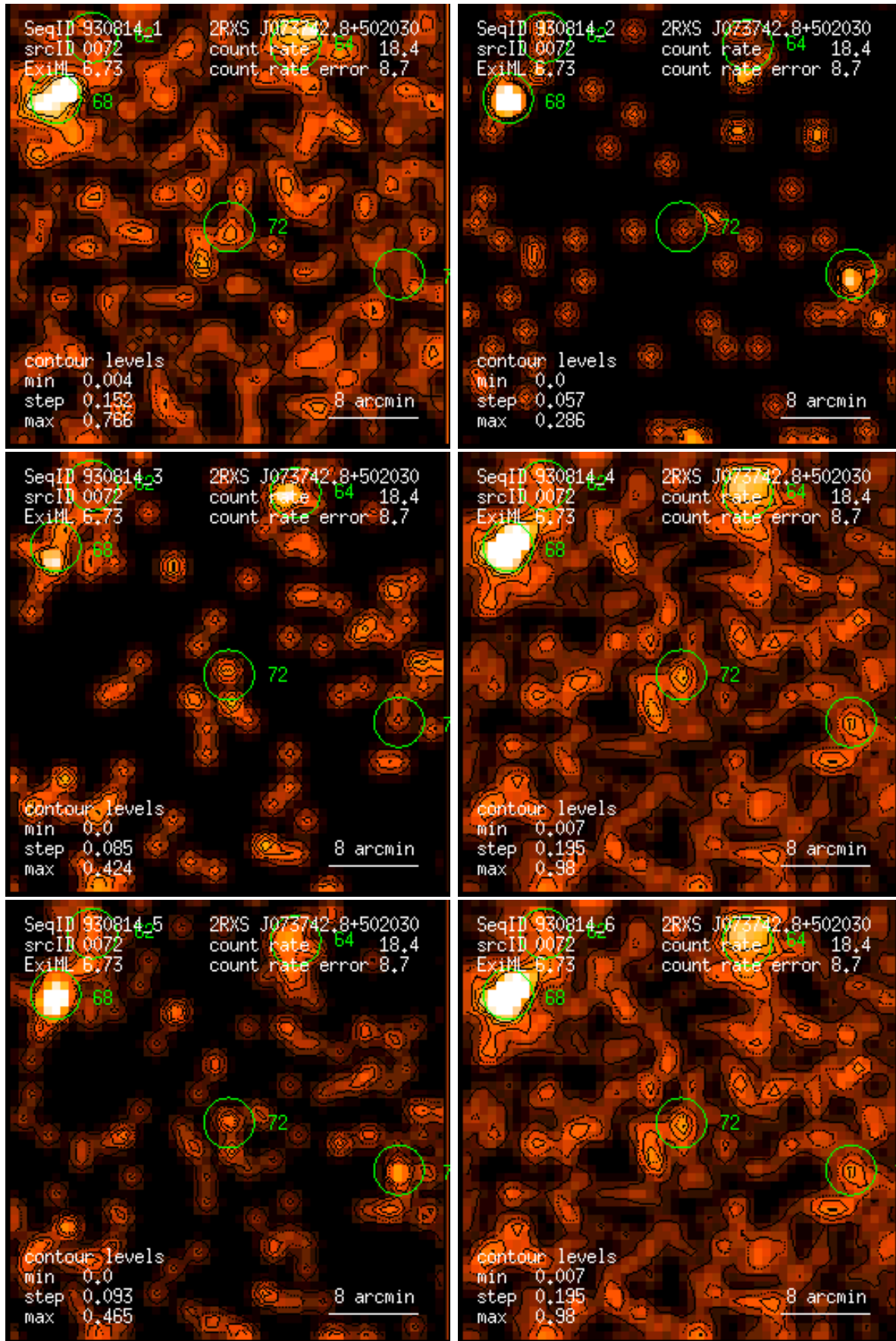
Figure 72: RASS 930814: detection 0072: band rate images, Gaussian filter: (1) PSPC channels 11 – 41, (2) 52 – 90, (3) 91 – 201, (4) 11 – 235, (5) 52 – 201, (6) 11 – 201. Broad band rates in counts/ks. Band rate contour levels in counts/ks/arcmin 2 .
