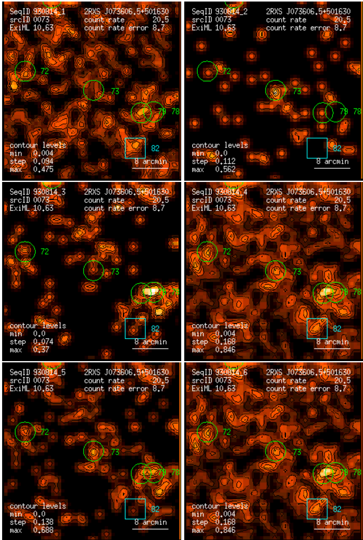
Figure 73: RASS 930814: detection 0073: band rate images, Gaussian filter: (1) PSPC channels 11 – 41, (2) 52 – 90, (3) 91 – 201, (4) 11 – 235, (5) 52 – 201, (6) 11 – 201. Broad band rates in counts/ks. Band rate contour levels in counts/ks/arcmin 2 .
