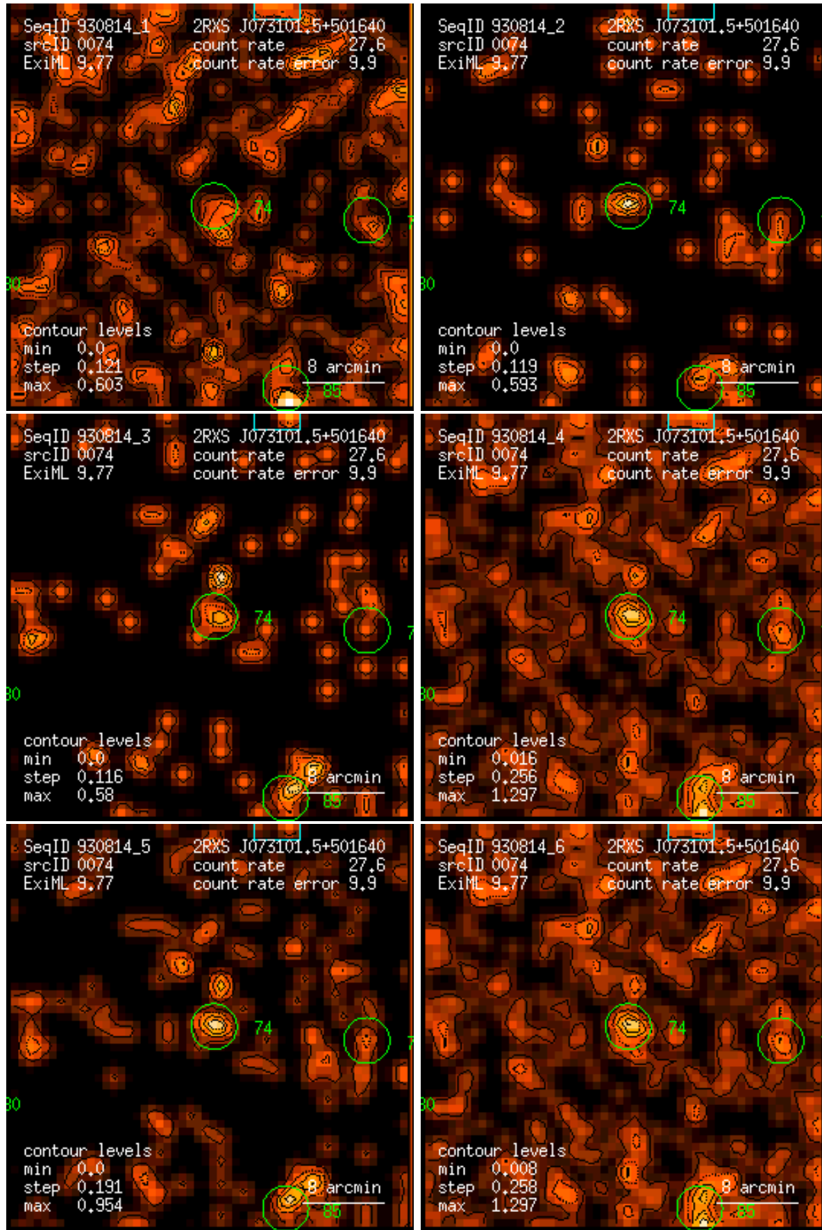
Figure 74: RASS 930814: detection 0074: band rate images, Gaussian filter: (1) PSPC channels 11 – 41, (2) 52 – 90, (3) 91 – 201, (4) 11 – 235, (5) 52 – 201, (6) 11 – 201. Broad band rates in counts/ks. Band rate contour levels in counts/ks/arcmin 2 .
