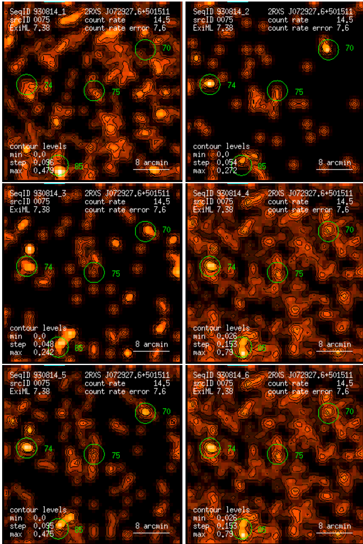
Figure 75: RASS 930814: detection 0075: band rate images, Gaussian filter: (1) PSPC channels 11 – 41, (2) 52 – 90, (3) 91 – 201, (4) 11 – 235, (5) 52 – 201, (6) 11 – 201. Broad band rates in counts/ks. Band rate contour levels in counts/ks/arcmin 2 .
