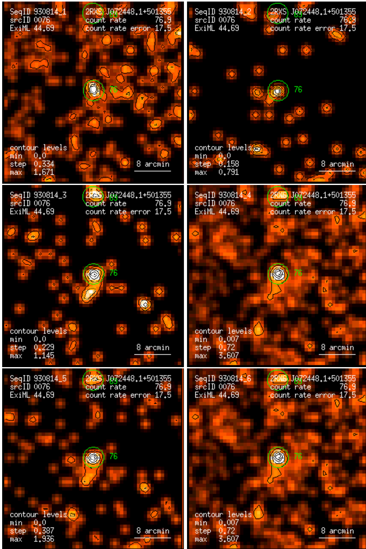
Figure 76: RASS 930814: detection 0076: band rate images, Gaussian filter: (1) PSPC channels 11 – 41, (2) 52 – 90, (3) 91 – 201, (4) 11 – 235, (5) 52 – 201, (6) 11 – 201. Broad band rates in counts/ks. Band rate contour levels in counts/ks/arcmin 2 .
