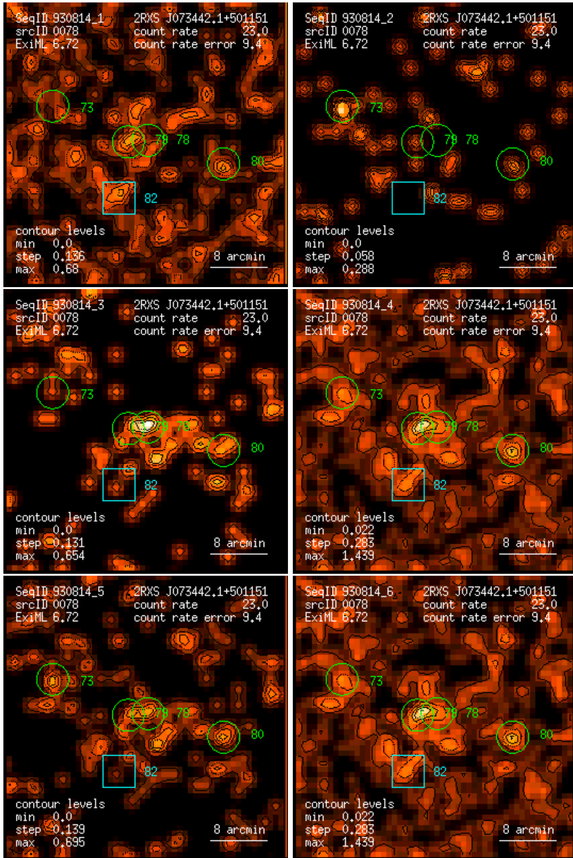
Figure 78: RASS 930814: detection 0078: band rate images, Gaussian filter: (1) PSPC channels 11 – 41, (2) 52 – 90, (3) 91 – 201, (4) 11 – 235, (5) 52 – 201, (6) 11 – 201. Broad band rates in counts/ks. Band rate contour levels in counts/ks/arcmin 2 .
