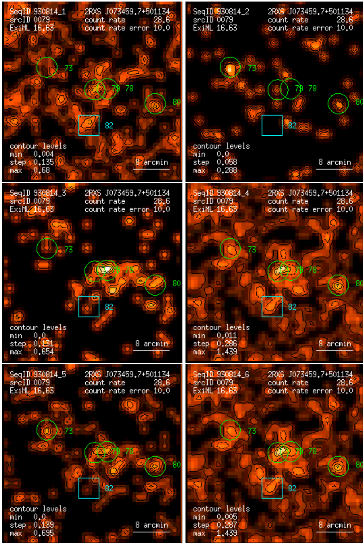
Figure 79: RASS 930814: detection 0079: band rate images, Gaussian filter: (1) PSPC channels 11 – 41, (2) 52 – 90, (3) 91 – 201, (4) 11 – 235, (5) 52 – 201, (6) 11 – 201. Broad band rates in counts/ks. Band rate contour levels in counts/ks/arcmin 2 .
