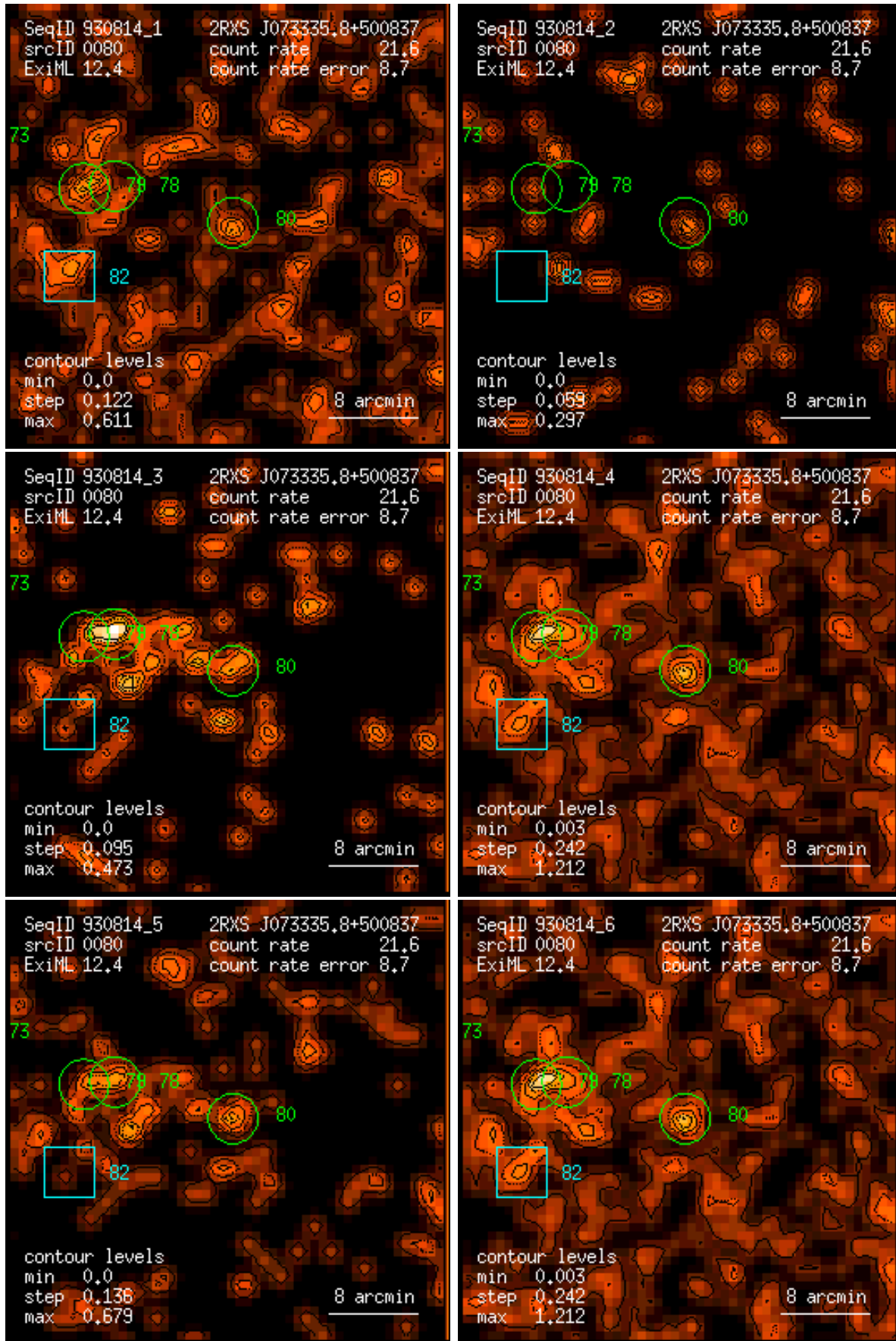
Figure 80: RASS 930814: detection 0080: band rate images, Gaussian filter: (1) PSPC channels 11 – 41, (2) 52 – 90, (3) 91 – 201, (4) 11 – 235, (5) 52 – 201, (6) 11 – 201. Broad band rates in counts/ks. Band rate contour levels in counts/ks/arcmin 2 .
