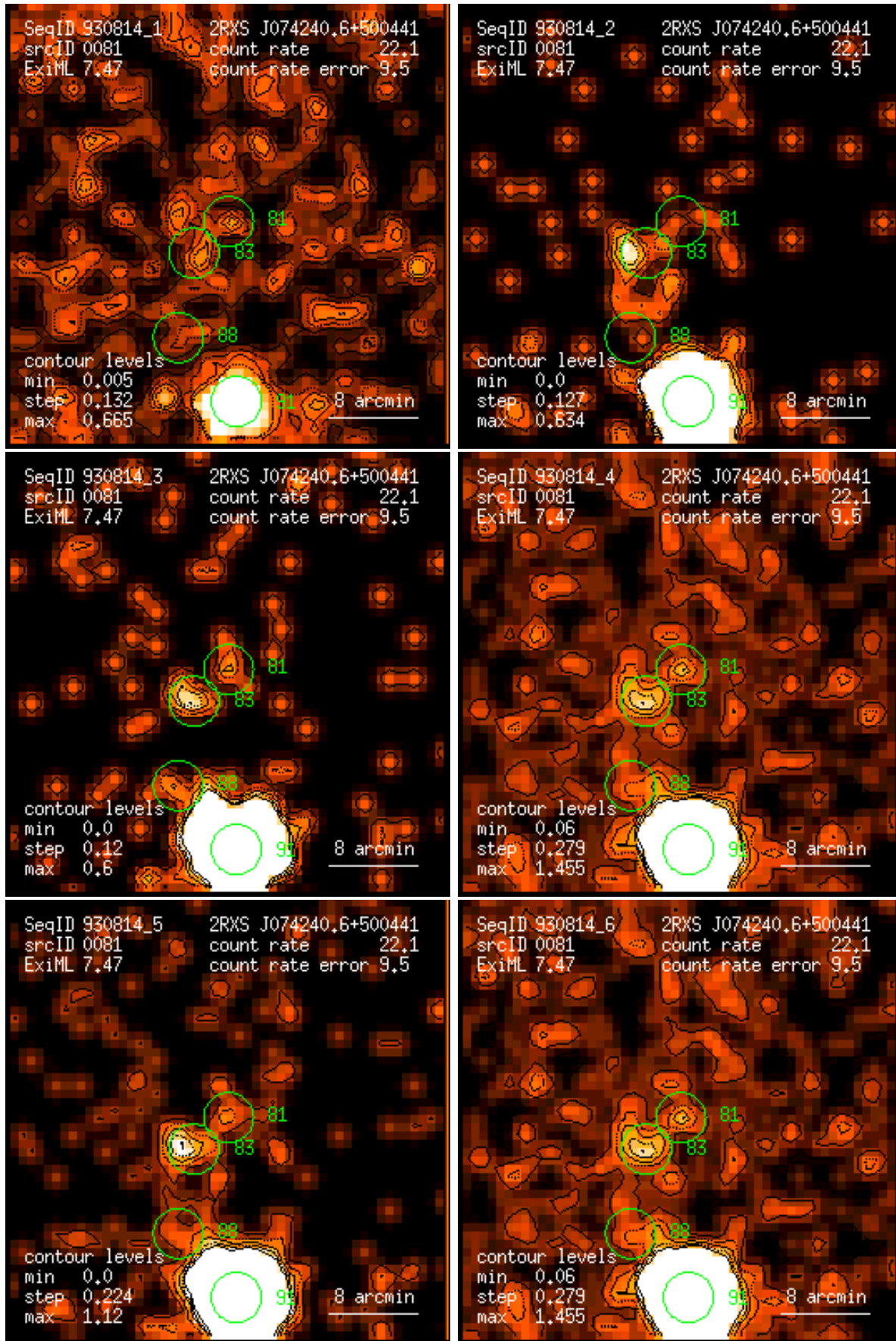
Figure 81: RASS 930814: detection 0081: band rate images, Gaussian filter: (1) PSPC channels 11 – 41, (2) 52 – 90, (3) 91 – 201, (4) 11 – 235, (5) 52 – 201, (6) 11 – 201. Broad band rates in counts/ks. Band rate contour levels in counts/ks/arcmin 2 .
