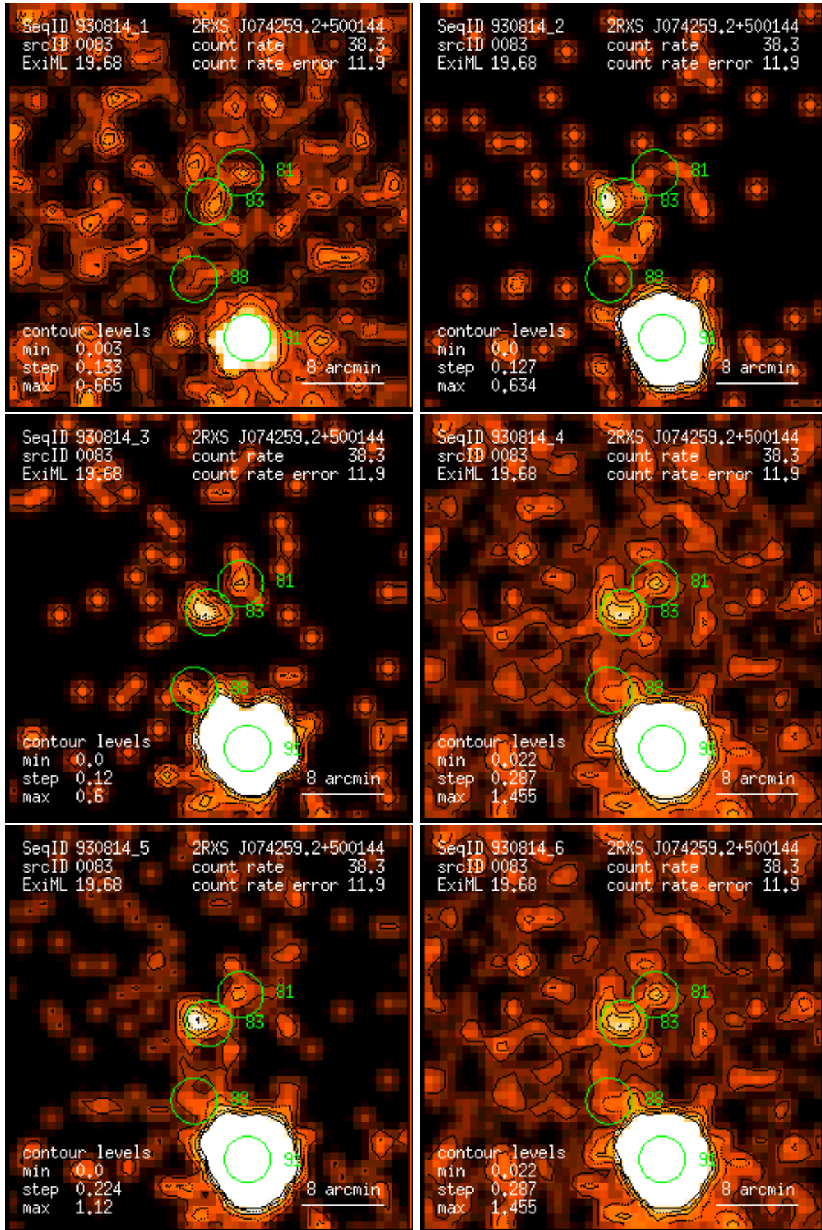
Figure 83: RASS 930814: detection 0083: band rate images, Gaussian filter: (1) PSPC channels 11 – 41, (2) 52 – 90, (3) 91 – 201, (4) 11 – 235, (5) 52 – 201, (6) 11 – 201. Broad band rates in counts/ks. Band rate contour levels in counts/ks/arcmin 2 .
