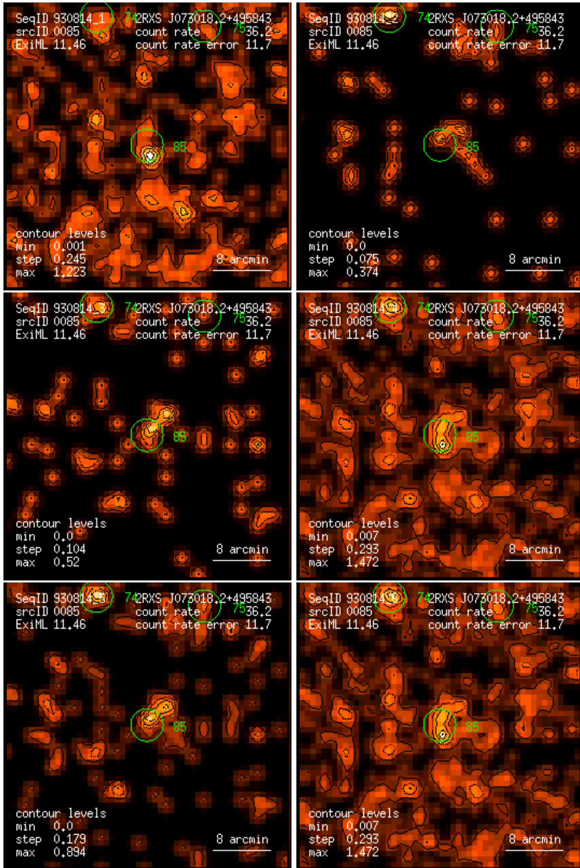
Figure 85: RASS 930814: detection 0085: band rate images, Gaussian filter: (1) PSPC channels 11 – 41, (2) 52 – 90, (3) 91 – 201, (4) 11 – 235, (5) 52 – 201, (6) 11 – 201. Broad band rates in counts/ks. Band rate contour levels in counts/ks/arcmin 2 .
