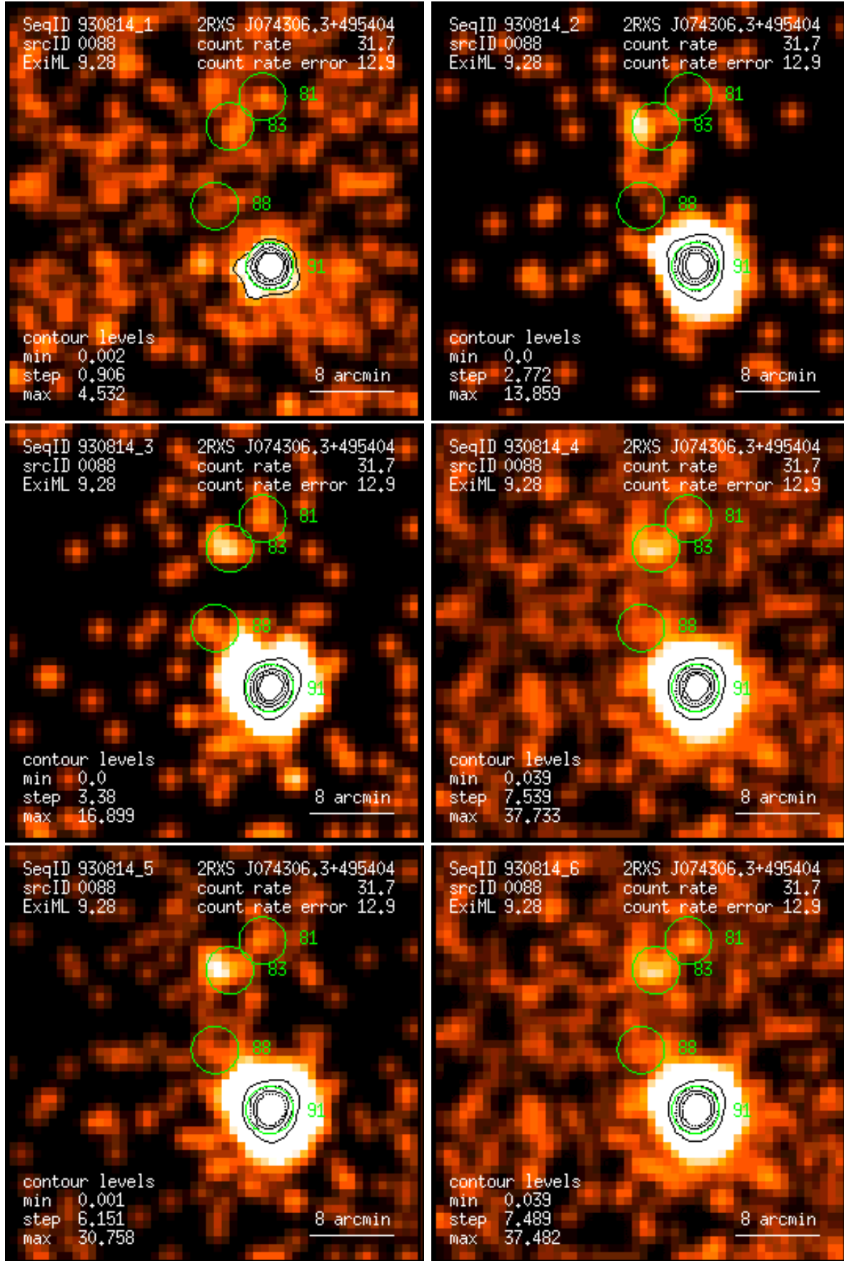
Figure 88: RASS 930814: detection 0088: band rate images, Gaussian filter: (1) PSPC channels 11 – 41, (2) 52 – 90, (3) 91 – 201, (4) 11 – 235, (5) 52 – 201, (6) 11 – 201. Broad band rates in counts/ks. Band rate contour levels in counts/ks/arcmin 2 .
