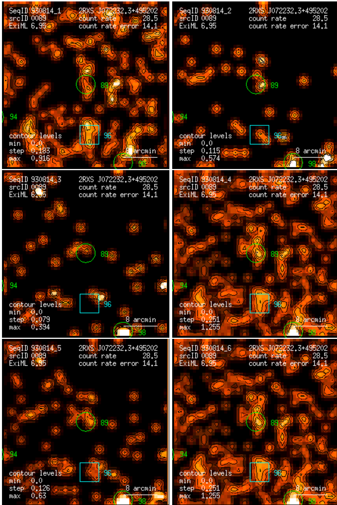
Figure 89: RASS 930814: detection 0089: band rate images, Gaussian filter: (1) PSPC channels 11 – 41, (2) 52 – 90, (3) 91 – 201, (4) 11 – 235, (5) 52 – 201, (6) 11 – 201. Broad band rates in counts/ks. Band rate contour levels in counts/ks/arcmin 2 .
