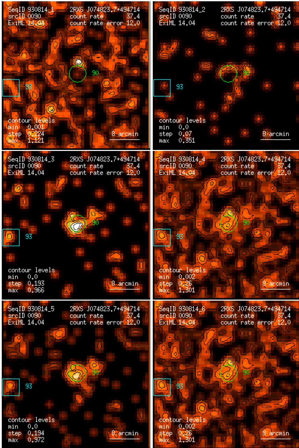
Figure 90: RASS 930814: detection 0090: band rate images, Gaussian filter: (1) PSPC channels 11 – 41, (2) 52 – 90, (3) 91 – 201, (4) 11 – 235, (5) 52 – 201, (6) 11 – 201. Broad band rates in counts/ks. Band rate contour levels in counts/ks/arcmin 2 .
