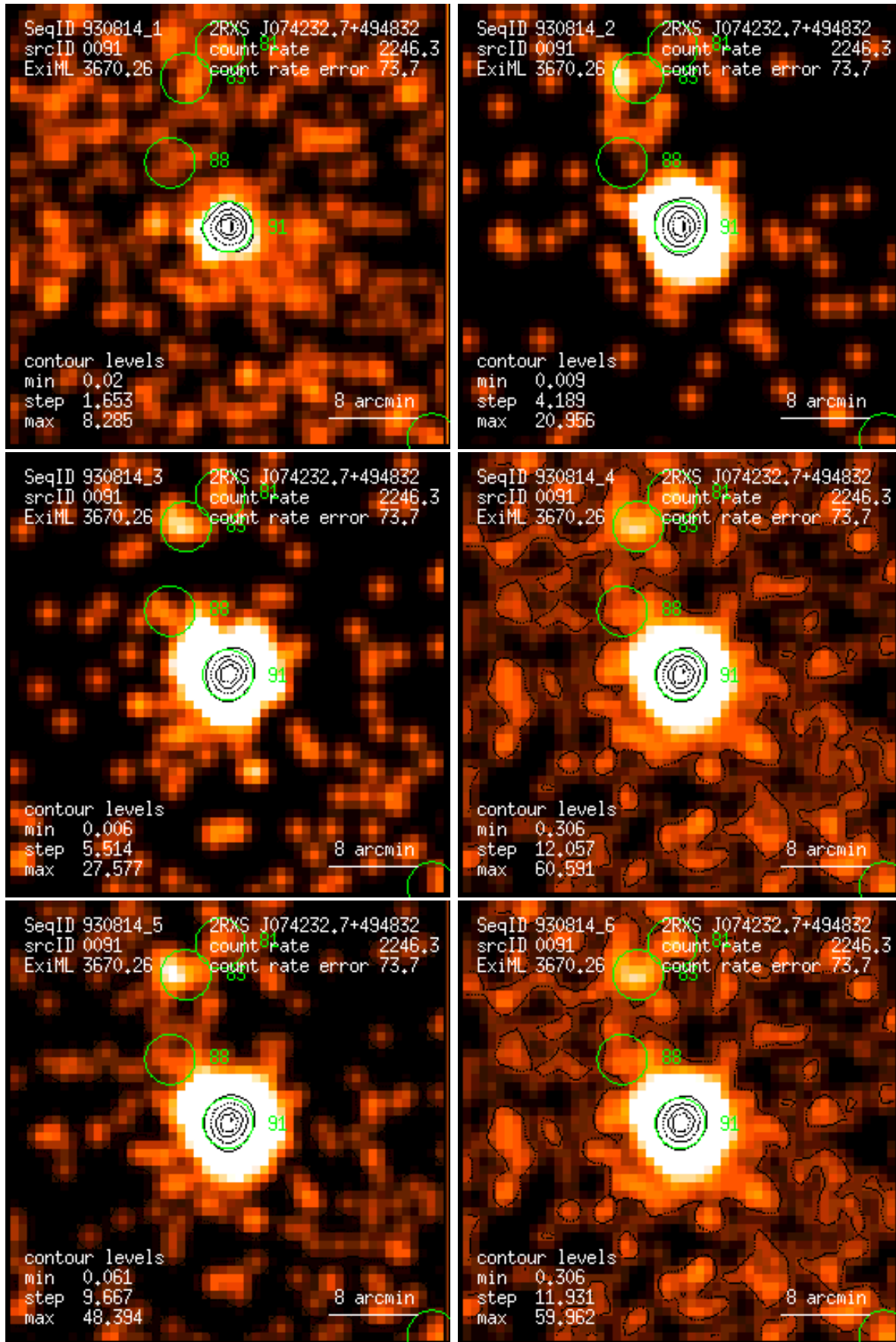
Figure 91: RASS 930814: detection 0091: band rate images, Gaussian filter: (1) PSPC channels 11 – 41, (2) 52 – 90, (3) 91 – 201, (4) 11 – 235, (5) 52 – 201, (6) 11 – 201. Broad band rates in counts/ks. Band rate contour levels in counts/ks/arcmin 2 .
