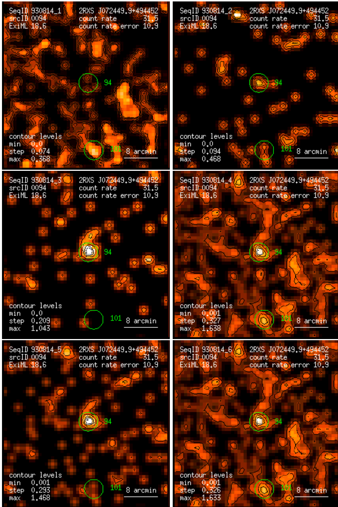
Figure 94: RASS 930814: detection 0094: band rate images, Gaussian filter: (1) PSPC channels 11 – 41, (2) 52 – 90, (3) 91 – 201, (4) 11 – 235, (5) 52 – 201, (6) 11 – 201. Broad band rates in counts/ks. Band rate contour levels in counts/ks/arcmin 2 .
