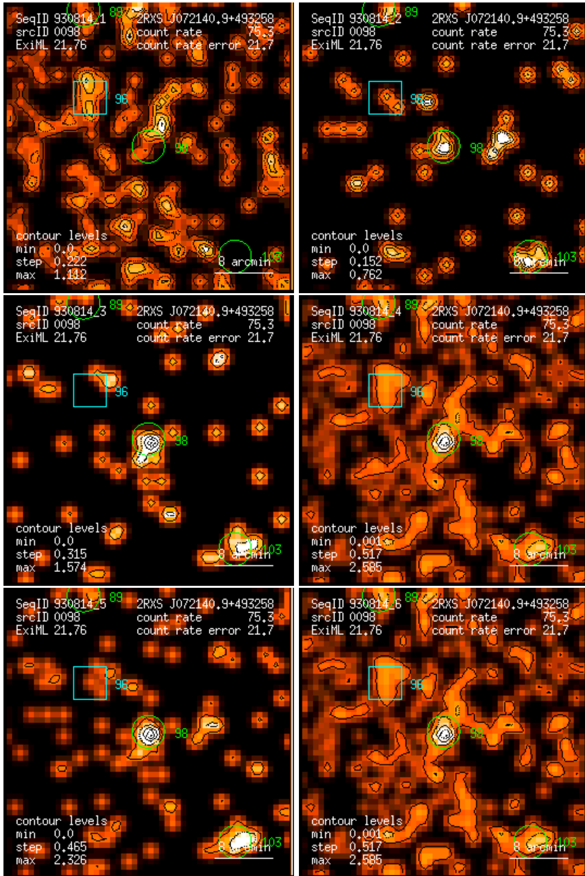
Figure 98: RASS 930814: detection 0098: band rate images, Gaussian filter: (1) PSPC channels 11 – 41, (2) 52 – 90, (3) 91 – 201, (4) 11 – 235, (5) 52 – 201, (6) 11 – 201. Broad band rates in counts/ks. Band rate contour levels in counts/ks/arcmin 2 .
