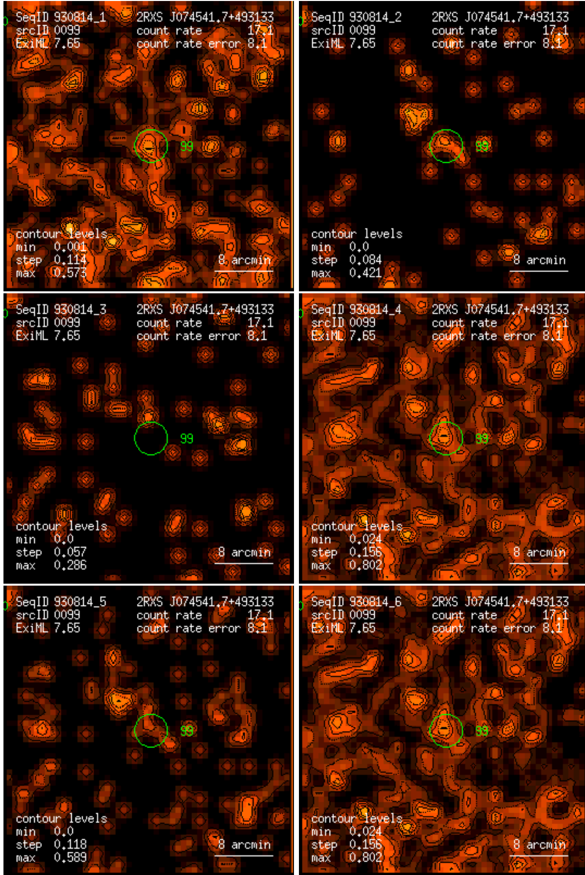
Figure 99: RASS 930814: detection 0099: band rate images, Gaussian filter: (1) PSPC channels 11 – 41, (2) 52 – 90, (3) 91 – 201, (4) 11 – 235, (5) 52 – 201, (6) 11 – 201. Broad band rates in counts/ks. Band rate contour levels in counts/ks/arcmin 2 .
