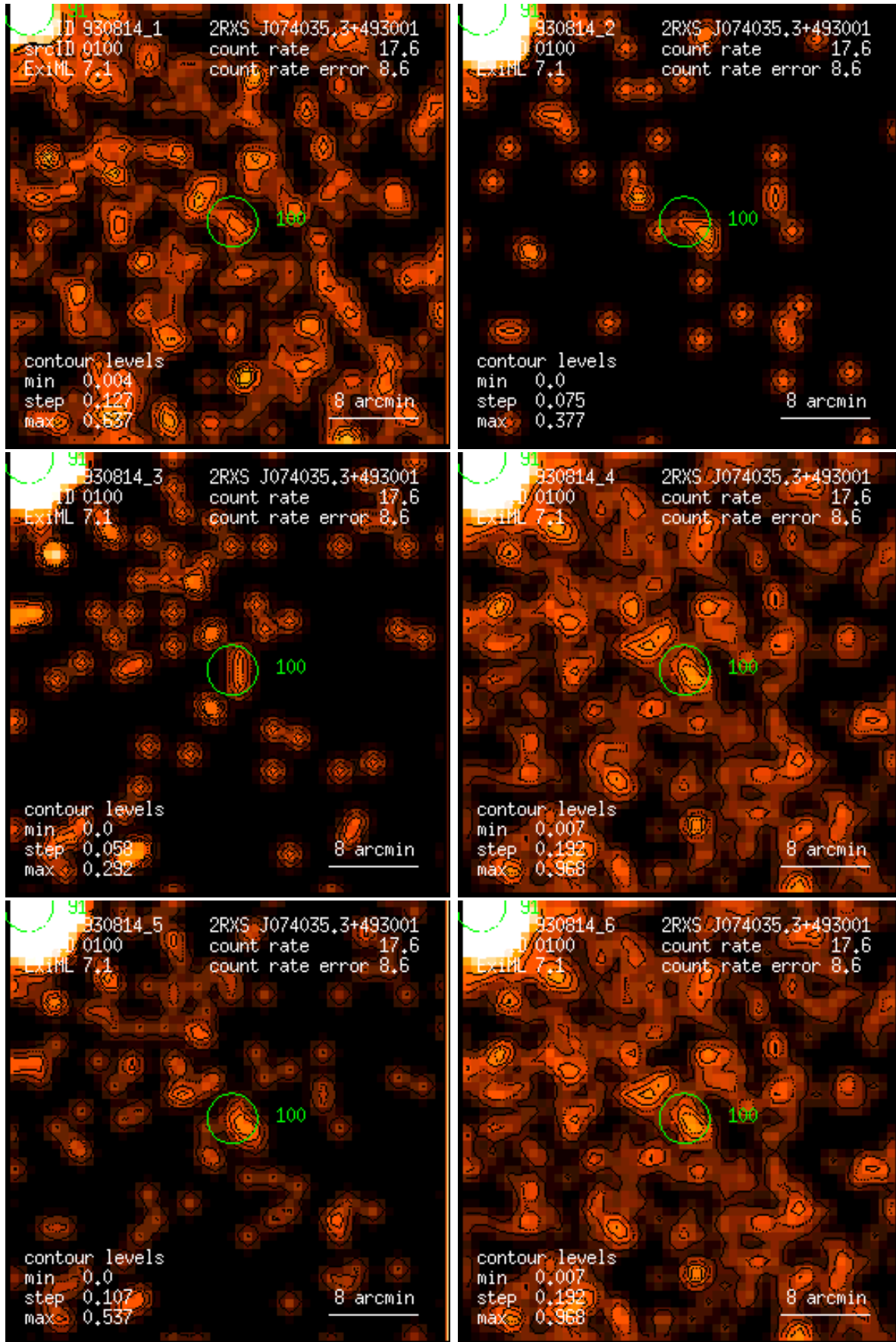
Figure 100: RASS 930814: detection 0100: band rate images, Gaussian filter: (1) PSPC channels 11 – 41, (2) 52 – 90, (3) 91 – 201, (4) 11 – 235, (5) 52 – 201, (6) 11 – 201. Broad band rates in counts/ks. Band rate contour levels in counts/ks/arcmin 2 .
