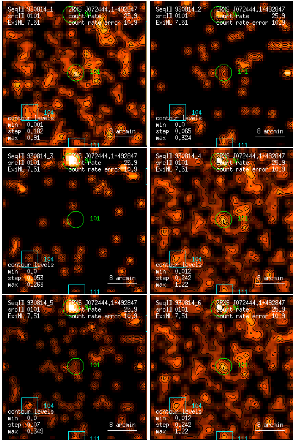
Figure 101: RASS 930814: detection 0101: band rate images, Gaussian filter: (1) PSPC channels 11 – 41, (2) 52 – 90, (3) 91 – 201, (4) 11 – 235, (5) 52 – 201, (6) 11 – 201. Broad band rates in counts/ks. Band rate contour levels in counts/ks/arcmin 2 .
