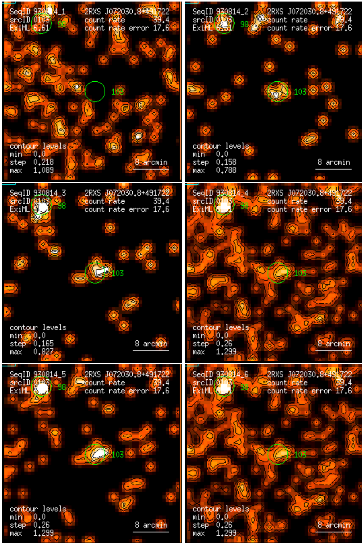
Figure 103: RASS 930814: detection 0103: band rate images, Gaussian filter: (1) PSPC channels 11 – 41, (2) 52 – 90, (3) 91 – 201, (4) 11 – 235, (5) 52 – 201, (6) 11 – 201. Broad band rates in counts/ks. Band rate contour levels in counts/ks/arcmin 2 .
