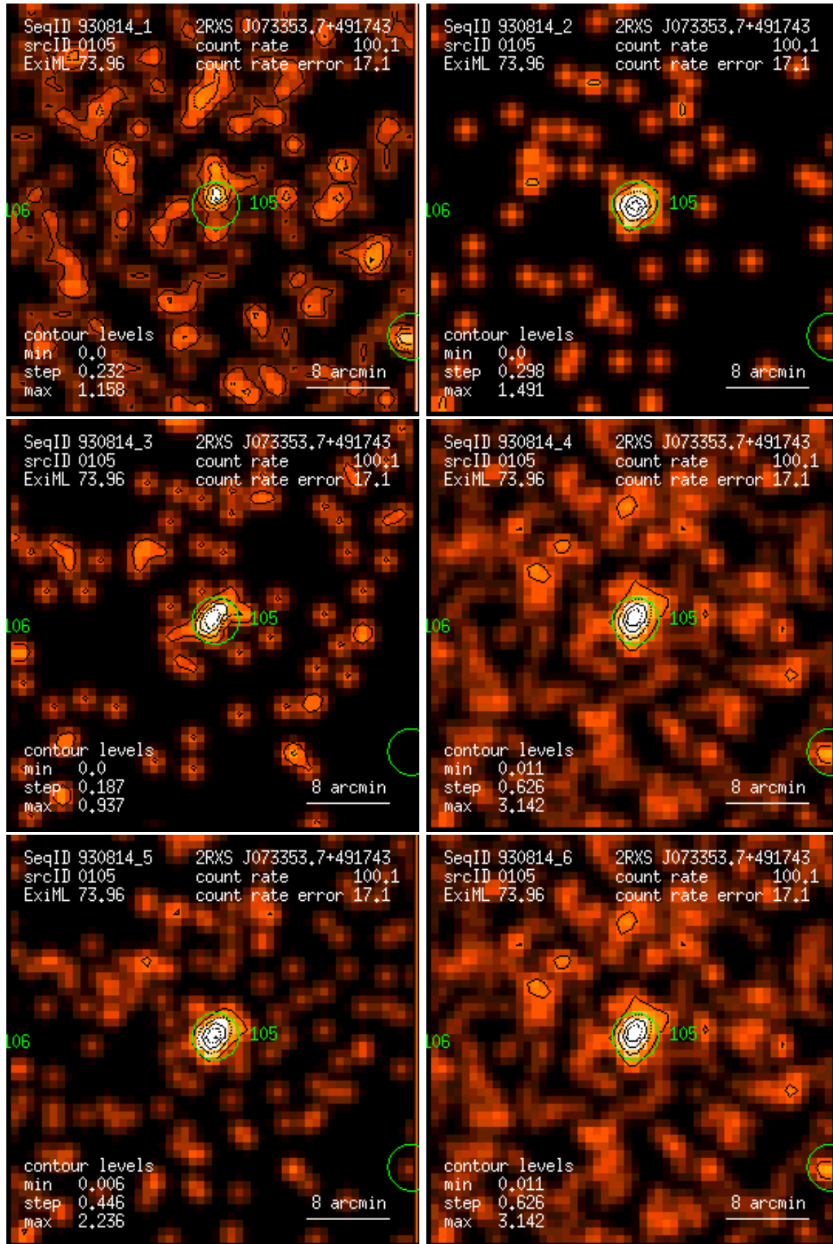
Figure 105: RASS 930814: detection 0105: band rate images, Gaussian filter: (1) PSPC channels 11 – 41, (2) 52 – 90, (3) 91 – 201, (4) 11 – 235, (5) 52 – 201, (6) 11 – 201. Broad band rates in counts/ks. Band rate contour levels in counts/ks/arcmin 2 .
