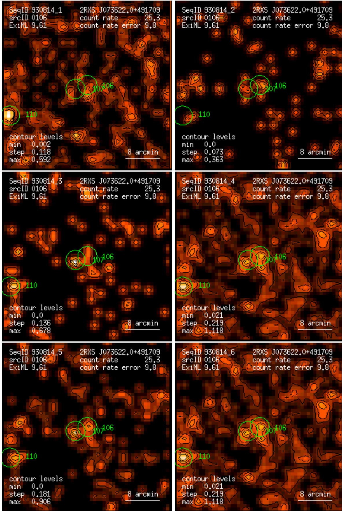
Figure 106: RASS 930814: detection 0106: band rate images, Gaussian filter: (1) PSPC channels 11 – 41, (2) 52 – 90, (3) 91 – 201, (4) 11 – 235, (5) 52 – 201, (6) 11 – 201. Broad band rates in counts/ks. Band rate contour levels in counts/ks/arcmin 2 .
